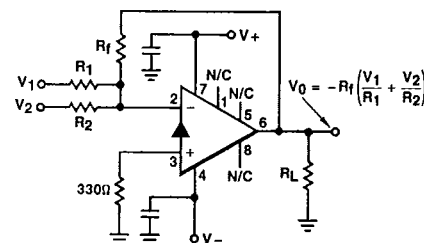
Summing Amplifier
