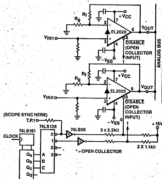
Using The EL2020 as a Multiplexer
