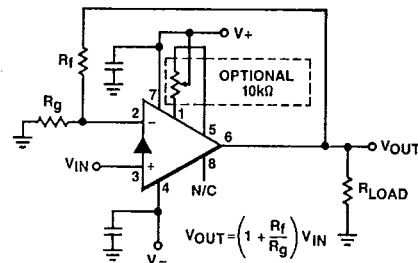
Non-Inverting Amplifier
