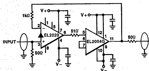
EL2020 Buffered With An EL2004
