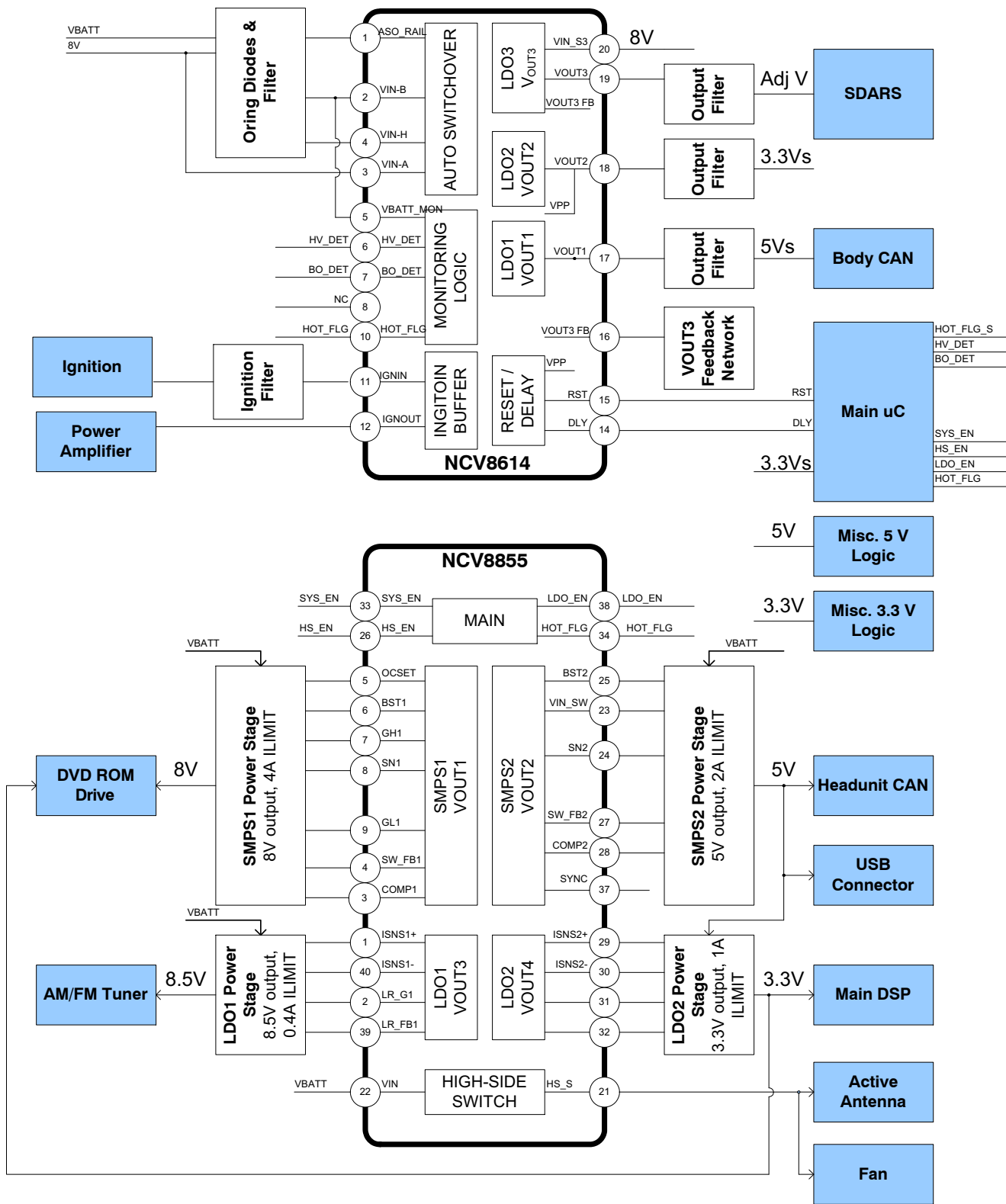
Figure 2. Automotive Radio System Block Diagram Example NCV8614 with NCV8855
