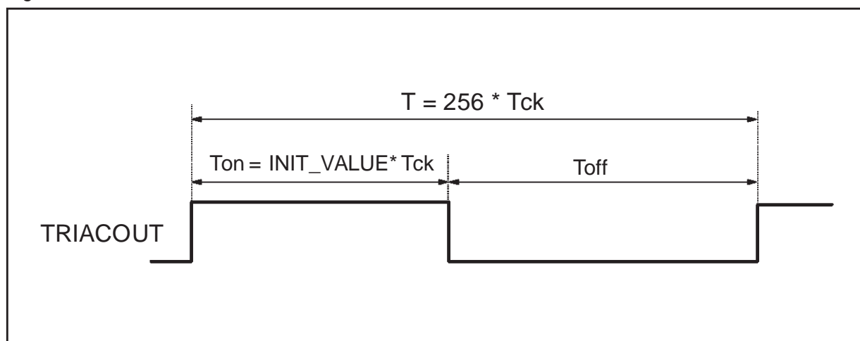
Figure 10.3. PWM Functionament
