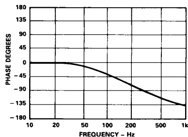
Figure 5. Phase Plot
