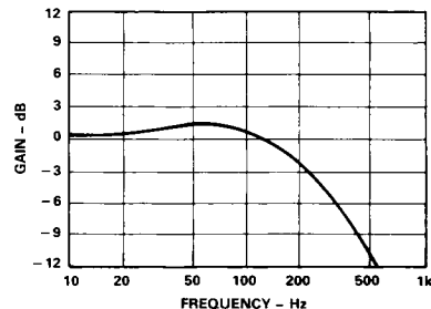
Figure 4. Gain Plot
