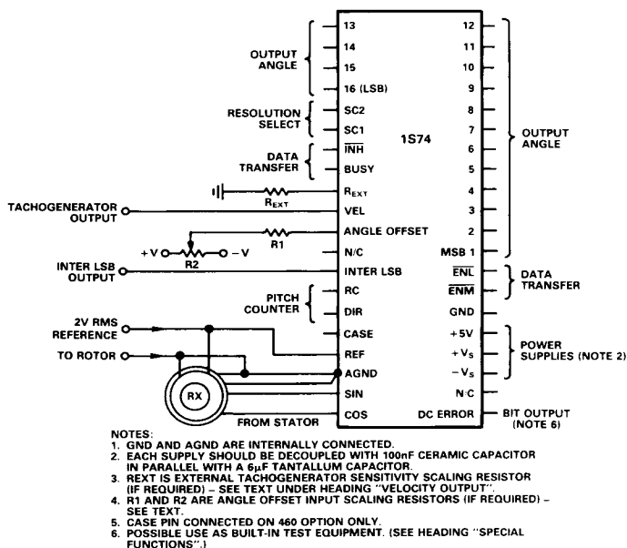
Figure 6. Electrical Connections
