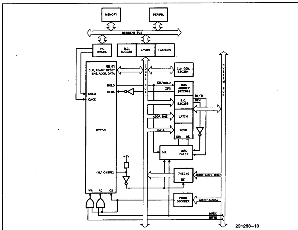
Figure 11. 82258 in Remote Mode
