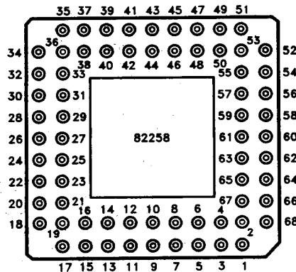
Figure 2. Pin Configuration in 286 Mode
