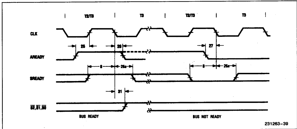
Figure 40. READY Timing (186 Mode)
