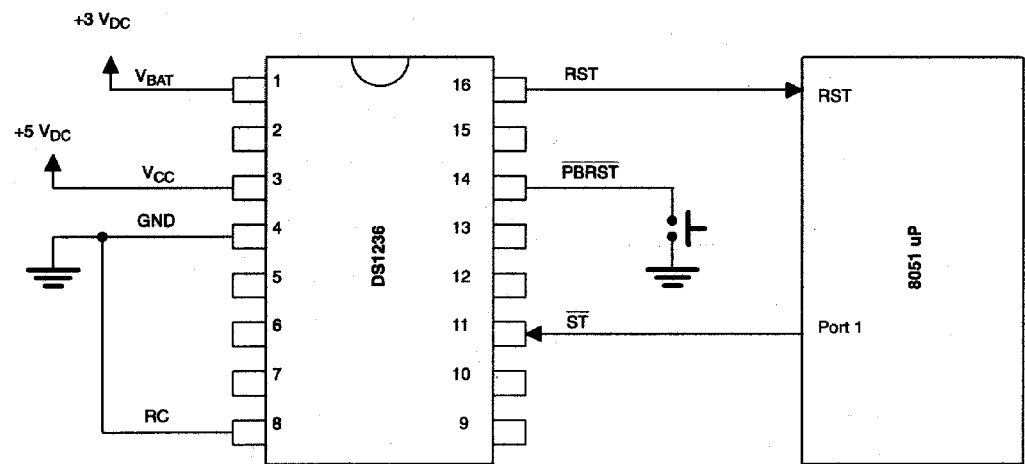
POWER MONITOR, WATCHDOG Figure 4
