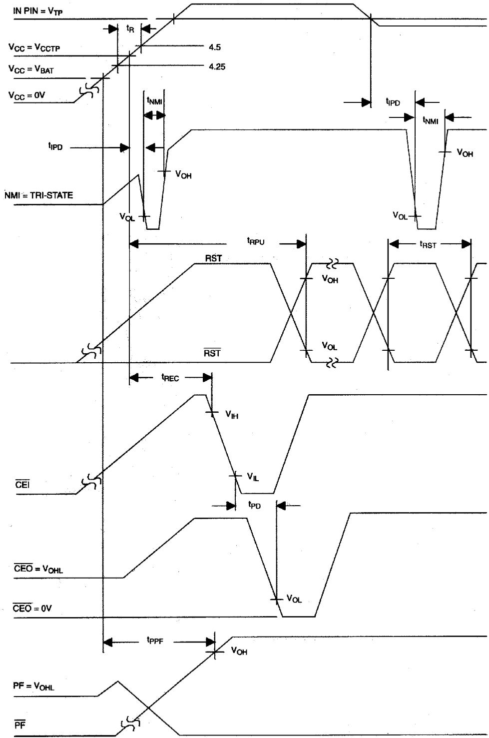
NMOS MODE POWER-UP (RC = GND) Figure 12
