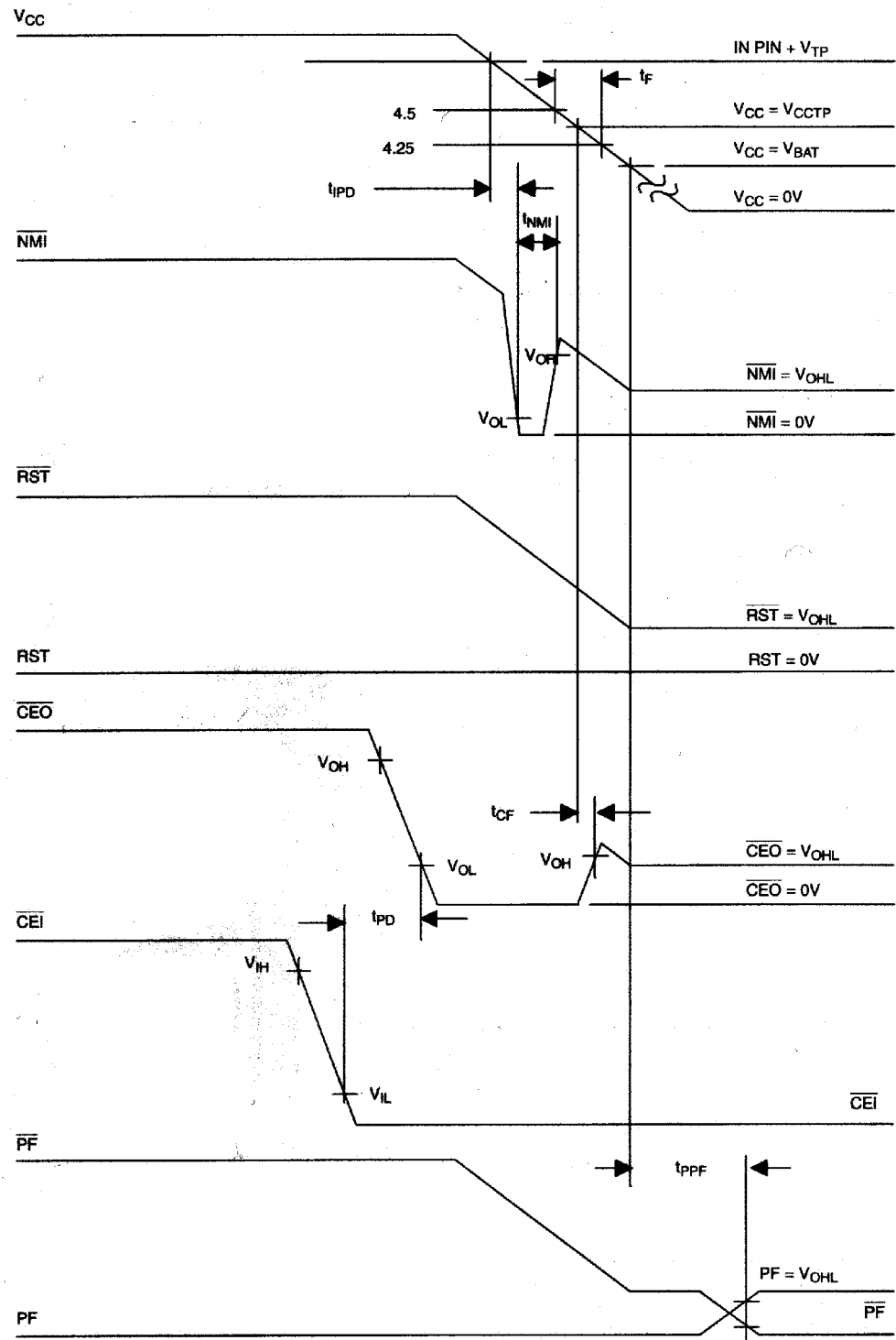
CMOS MODE POWER-DOWN ( R_C = V_{CC0} ) Figure 10
