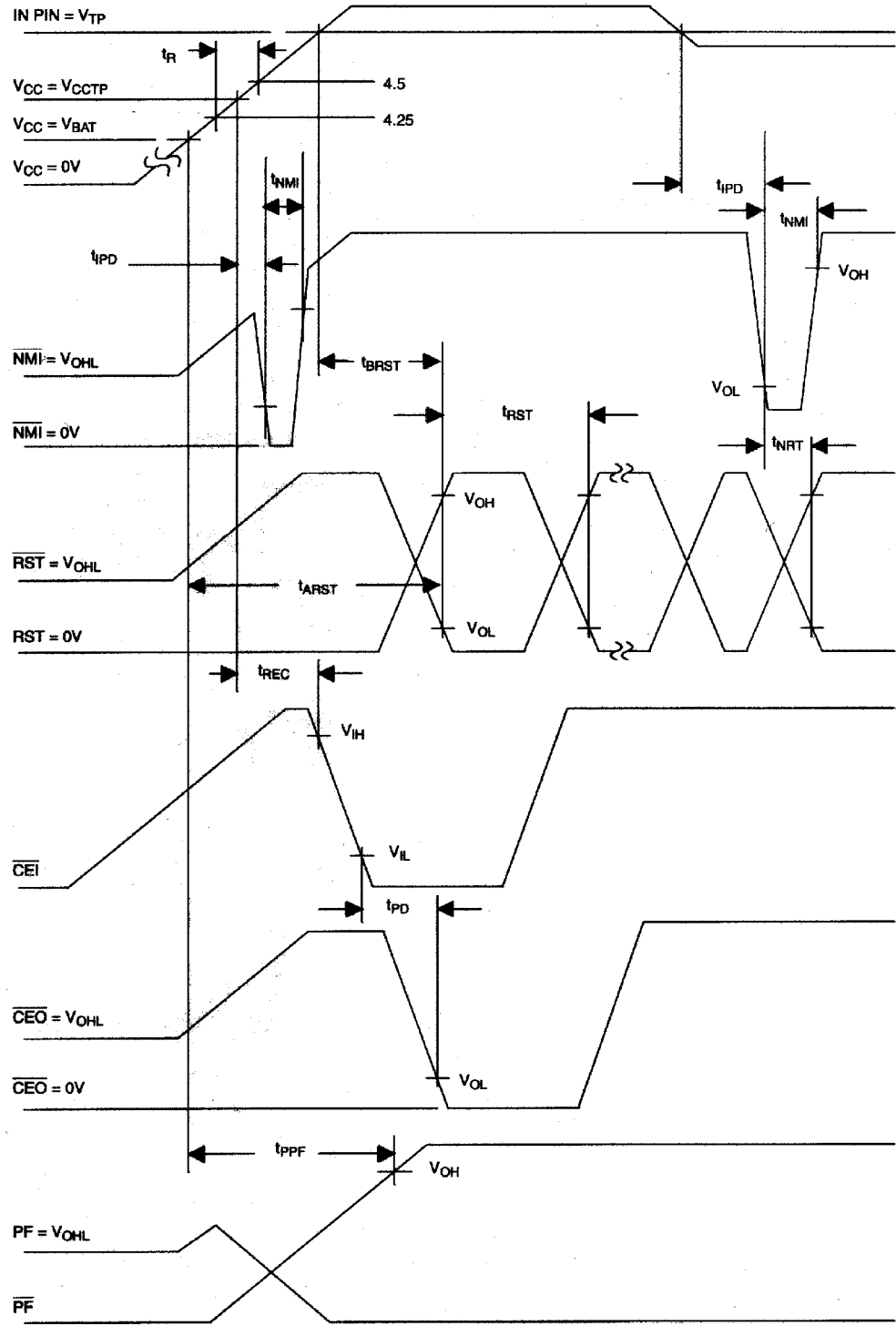
CMOS MODE POWER-UP (RC = V CCO ) Figure 13
