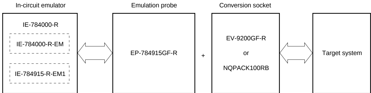
Figure 1-1. Connection of IE-784000-R and Target System
