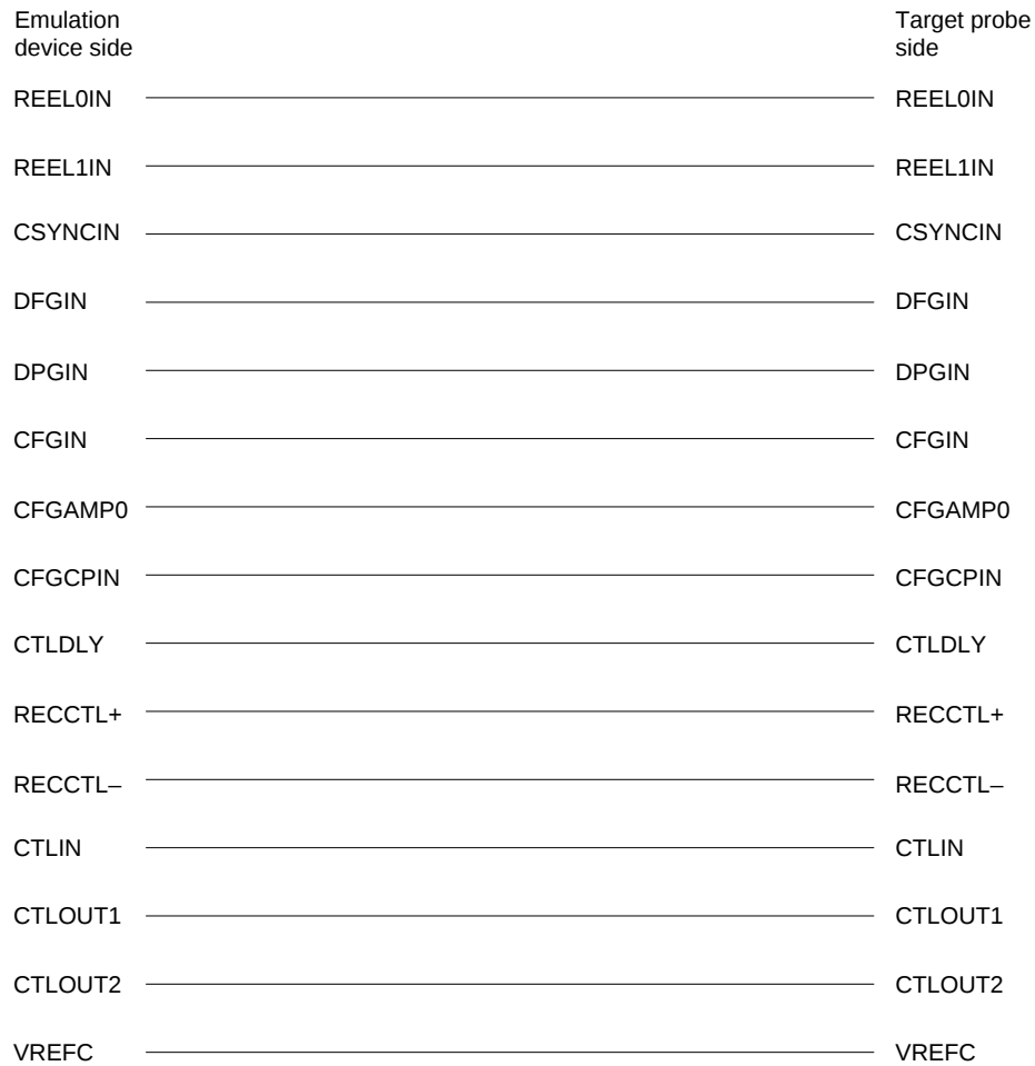
Figure 5-1. Equivalent Circuit Diagram of Port Pin Emulation Circuit (3/3)
