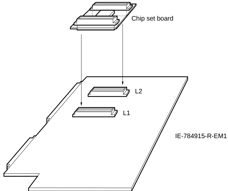
Figure 2-2. Connection of Chip Set Board
