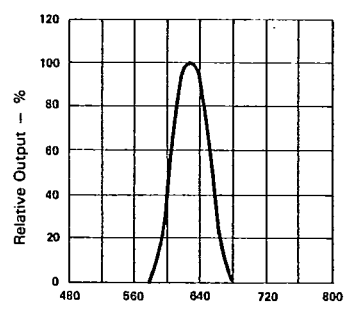
Fig. 2 SPECTRAL RESPONSE.
