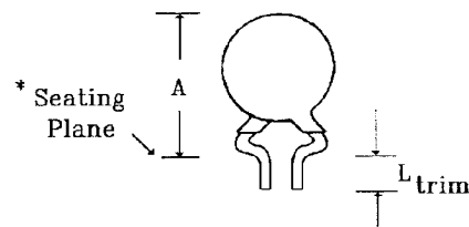
CRIMPED AND TRIMMED LEAD
