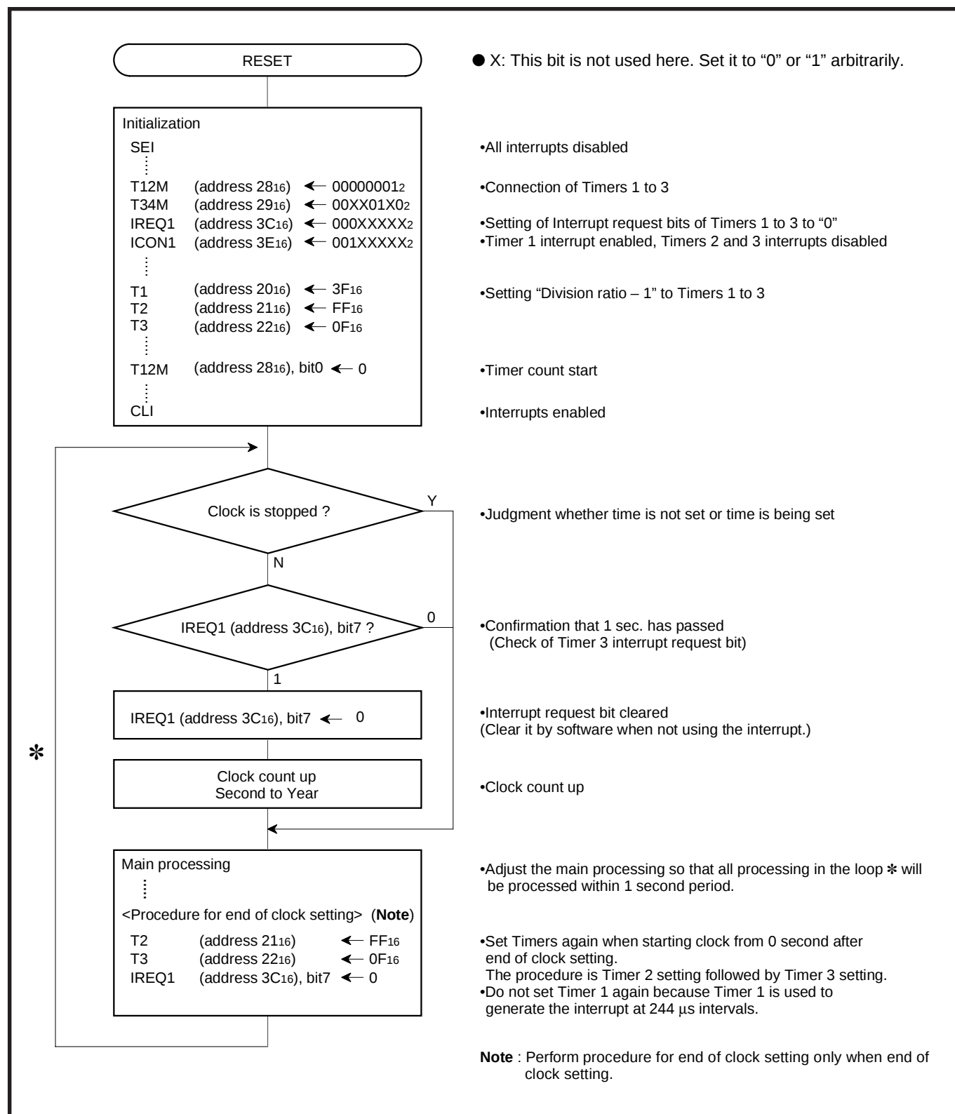
Fig. 2.2.18 Control procedure
