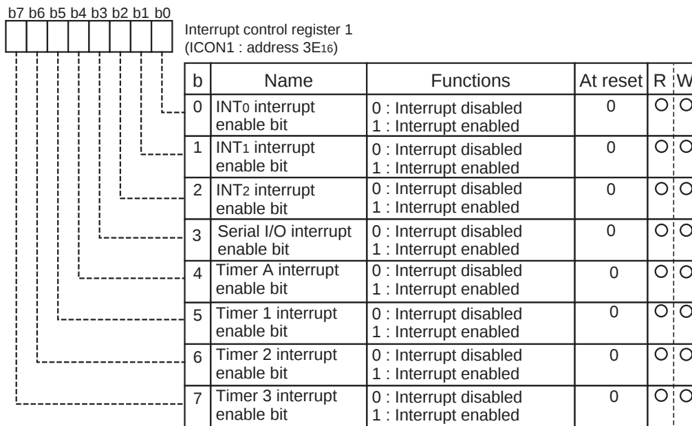
Fig. 3.5.32 Structure of Interrupt control register 1
