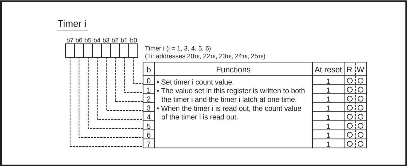
Fig. 2.2.2 Structure of Timer i (i=1, 3, 4, 5, 6)
