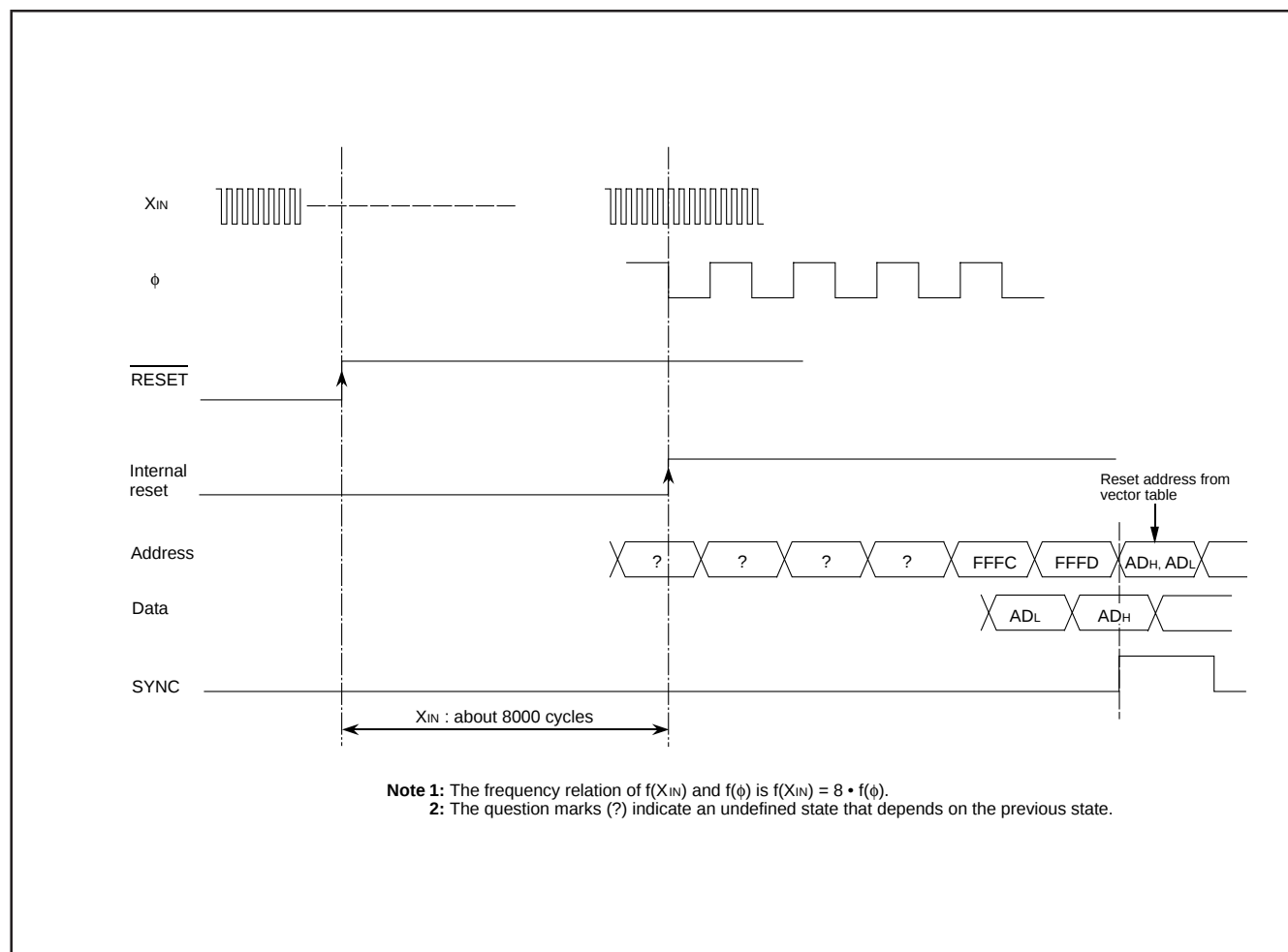
Fig. 40 Reset sequence
