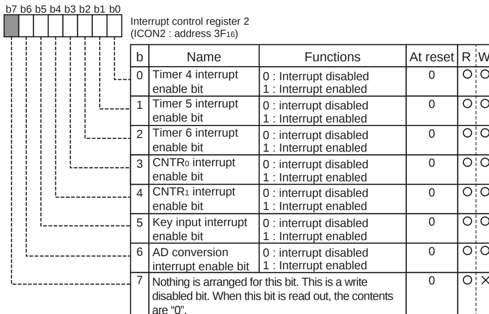
Fig. 3.5.33 Structure of Interrupt control register 2
