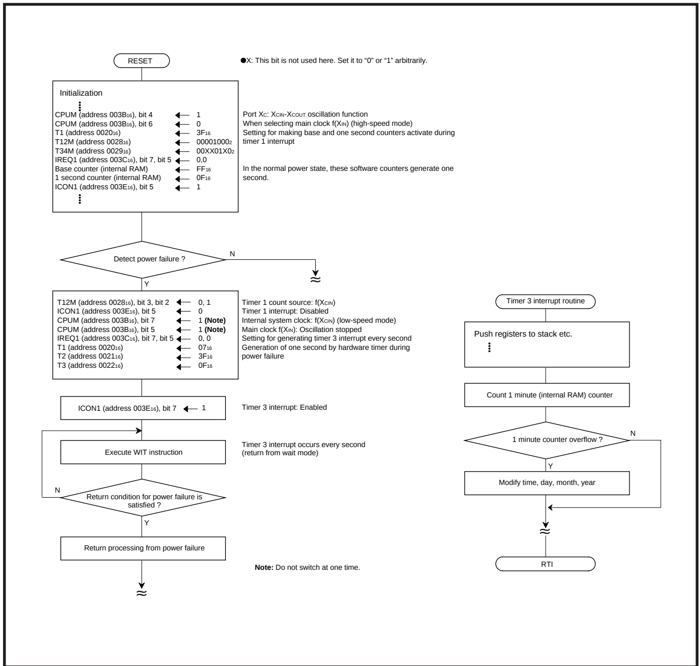
Fig. 2.8.9 Control procedure
