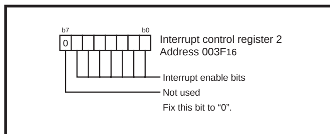
Fig. 3.3.3 Structure of interrupt control register 2
