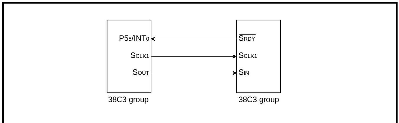
Fig. 2.3.9 Connection diagram
