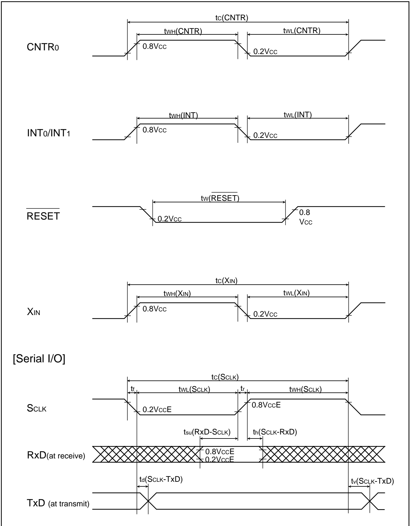
Fig. 144 Timing chart (1)
