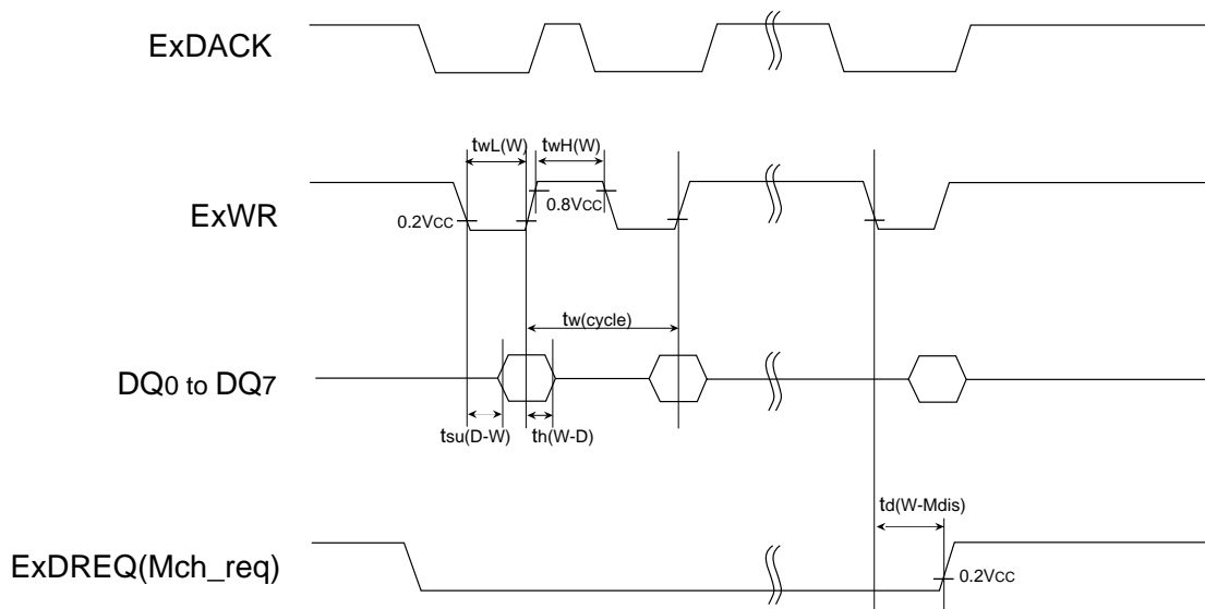
Fig. 149 Timing chart (6)
