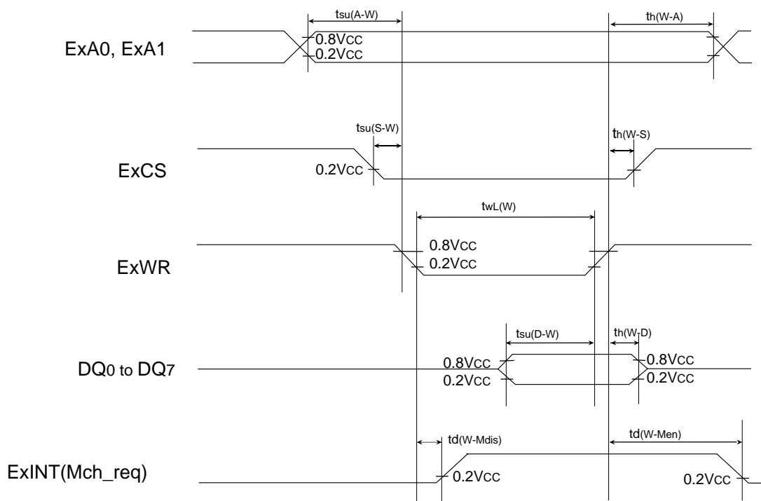
Fig. 146 Timing chart (3)
