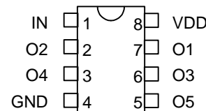
3D3215M-xx DIP (300 Mil)
