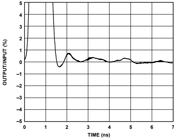
Figure 61. AD8117 Settling Time (Zoom)
