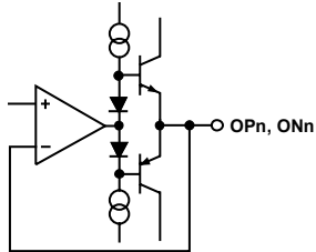
Figure 8. AD8117/AD8118 Enabled Output (see also ESD Protection Map, Figure 18)
