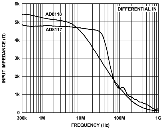
Figure 38. AD8117, AD8118 Input Impedance
