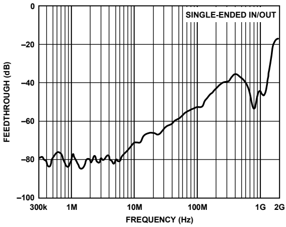
Figure 37. AD8117 Crosstalk, Off Isolation, Single-Ended
