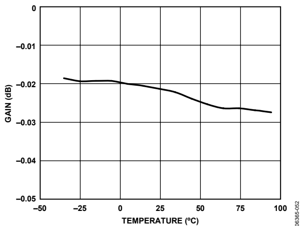
Figure 57. AD8117 DC Gain vs. Temperature
