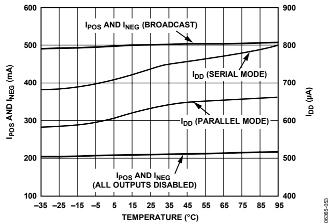
Figure 58. AD8117, AD8118 Quiescent Supply Currents vs. Temperature
