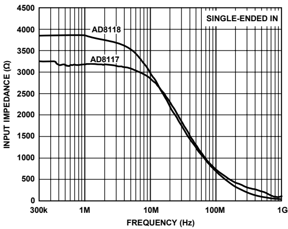
Figure 39. AD8117, AD8118 Input Impedance, Single-Ended
