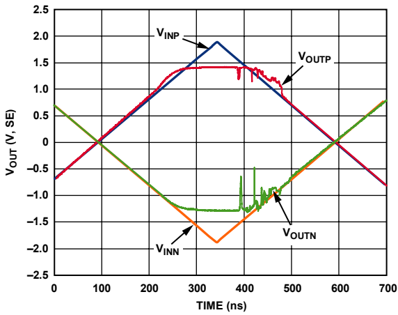
Figure 62. AD8117 Overdrive Recovery, Single-Ended
