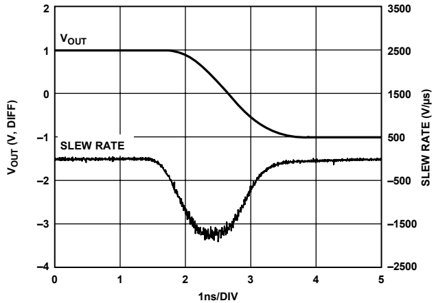
Figure 48. AD8117 Large Signal Falling Edge and Slew Rate
