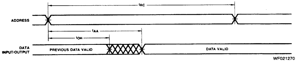
Read Cycle No. 1 ( \overline{WE} HIGH, \overline{CE} LOW)
