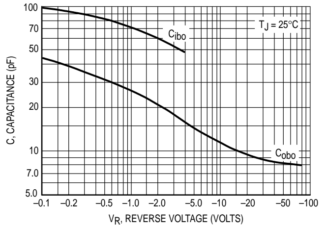
Figure 5. Capacitance
