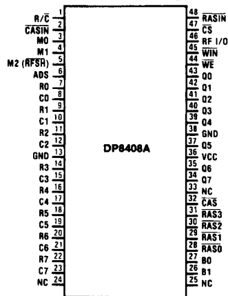
Dual In-Line Package
