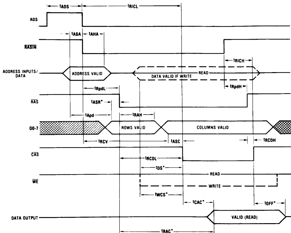
FIGURE 5a. Modes 5, 6 Timing (CASIN) High in Mode 6
