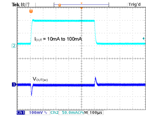
HT72B15 V_{IN}=2.5V , C_{IN}=C_{OUT}=1\mu F , CH1= V_{OUT(ac)} , CH2= I_{OUT}
