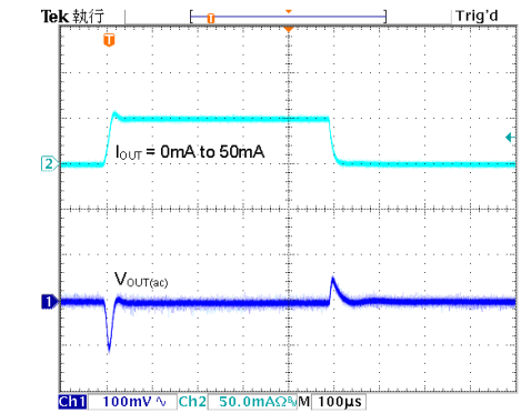
HT72B25 V_{IN}=3.5V , C_{IN}=C_{OUT}=1\mu F , CH1= V_{OUT(ac)} , CH2= I_{OUT}
