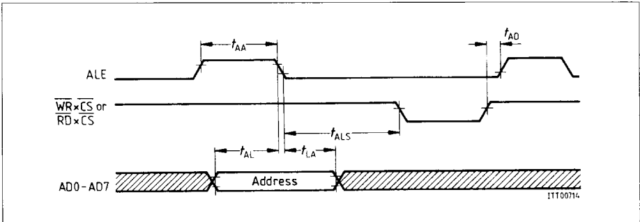
Figure 37 Multiplexed Address Timing
