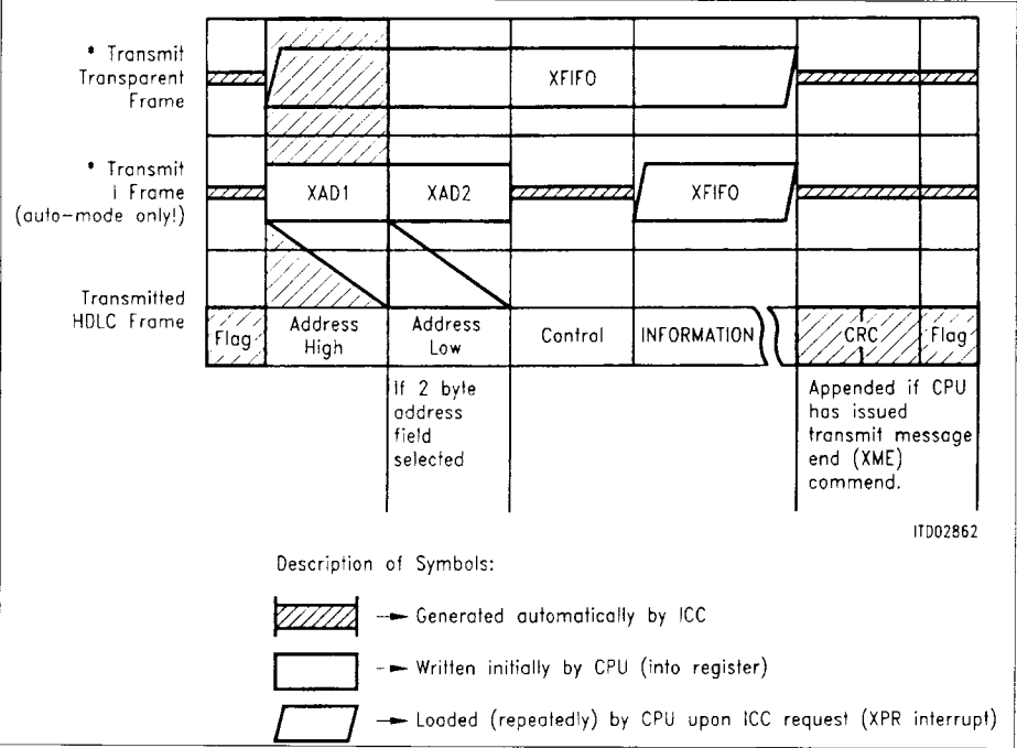
Figure 33 Transmit Data Flow
