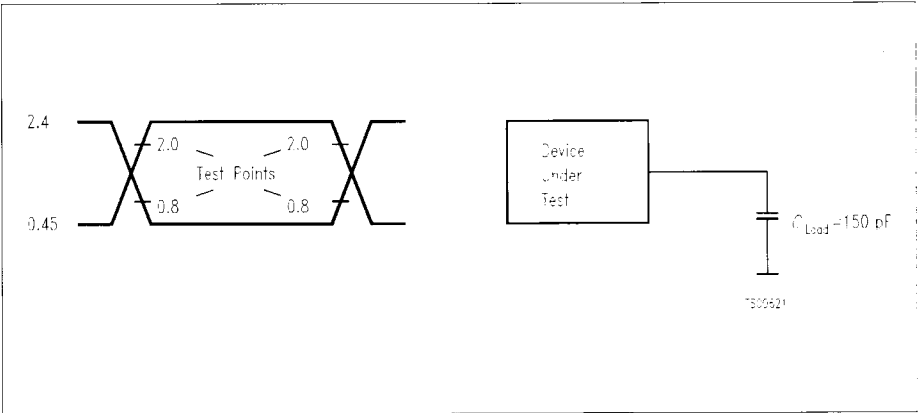
Input/Output Waveform and Load Circuit for AC Tests
