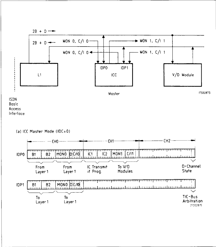
Figure 28 IOM® Data Ports 0, 1 in Terminal Mode (SPM = 0)
