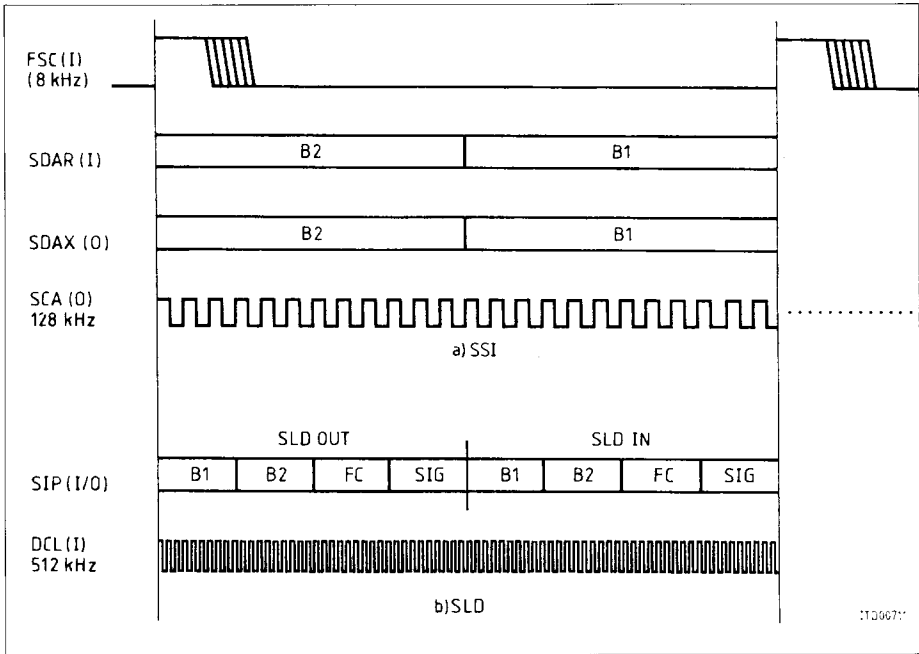
Figure 13 SSI (a) and SLD (b) Interface Lines
