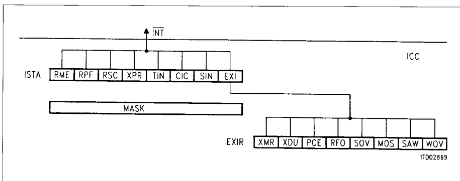
ICC Interrupt Structure
