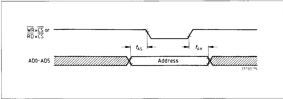
Figure 38 Non-Multiplexed Address Timing
