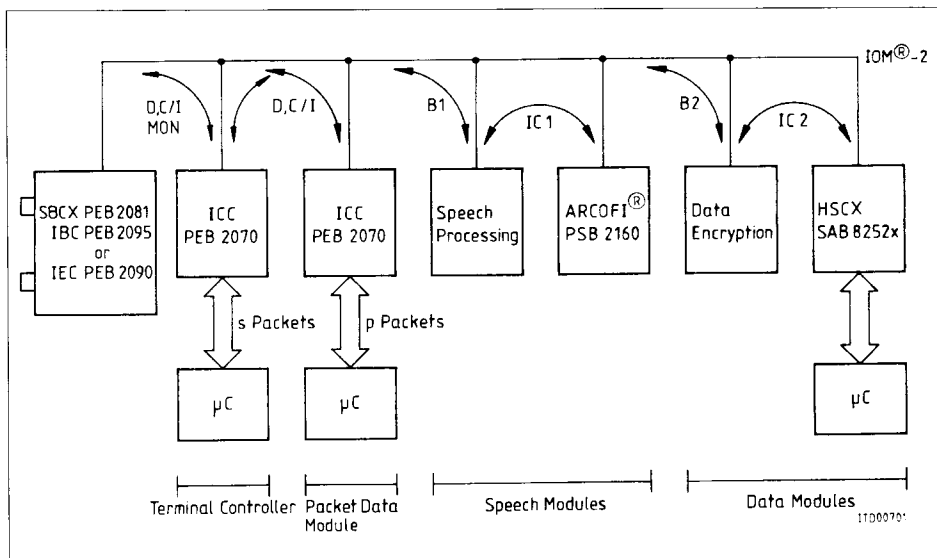
Figure 3 Example of ISDN Voice/ Data Terminal
