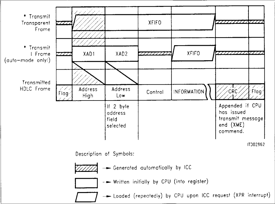
Figure 17 Transmit Data Flow
