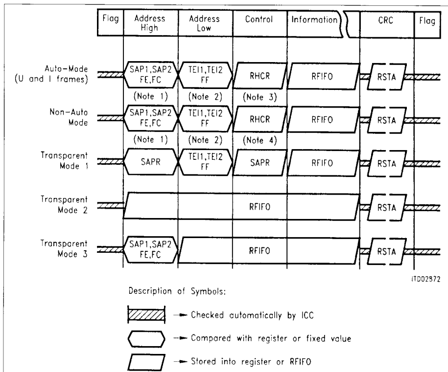
Figure 32 Receive Data Flow
