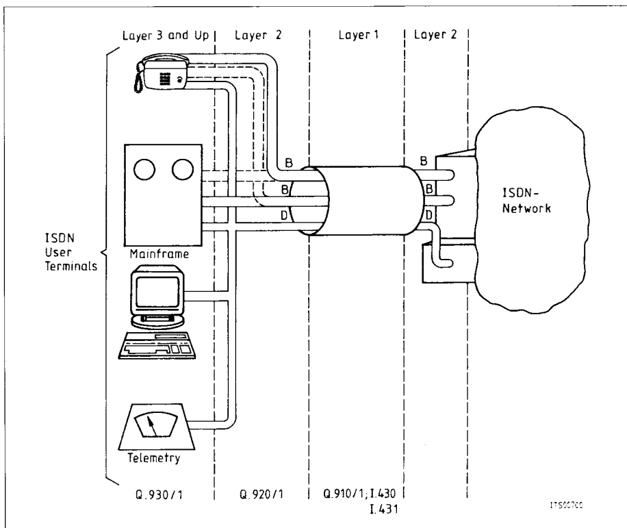
ISDN Basic Access Channel Structure
