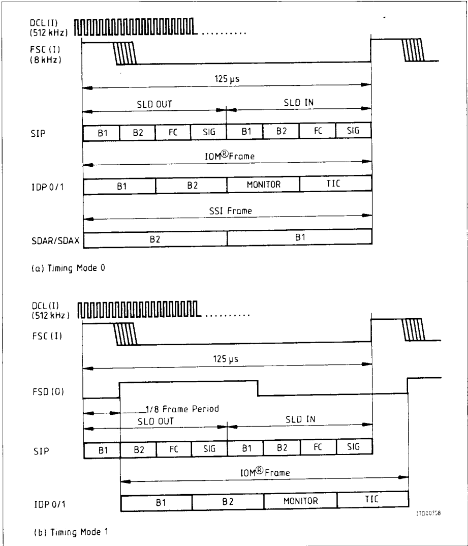
Figure 10 Interface Timing in IOM ® -1 Mode
