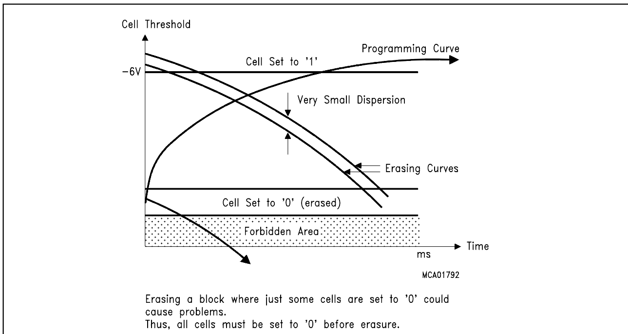
Figure 11 Flash Erasure
