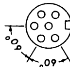
DIN 6 pin Fully Screened Line Socket. 2006
