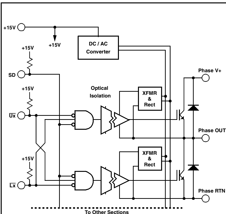
FIGURE 1 – BLOCK DIAGRAM
