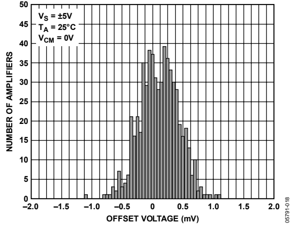
Figure 10. Input Offset Voltage Distribution, V_S = \pm 5 V
