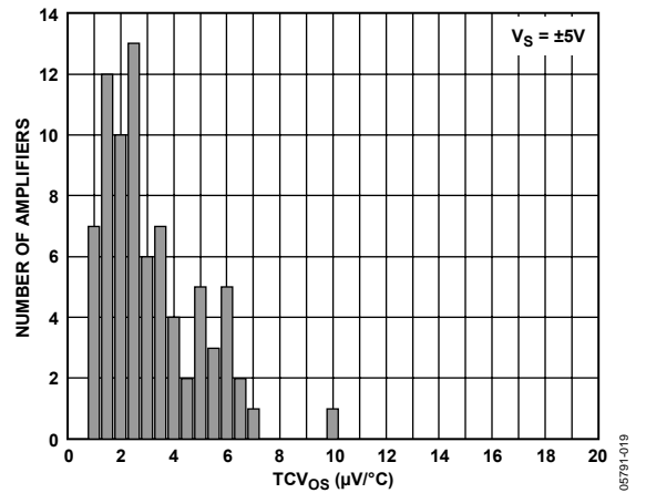
Figure 11. Offset Voltage Drift Distribution, V_S = \pm 5 V
