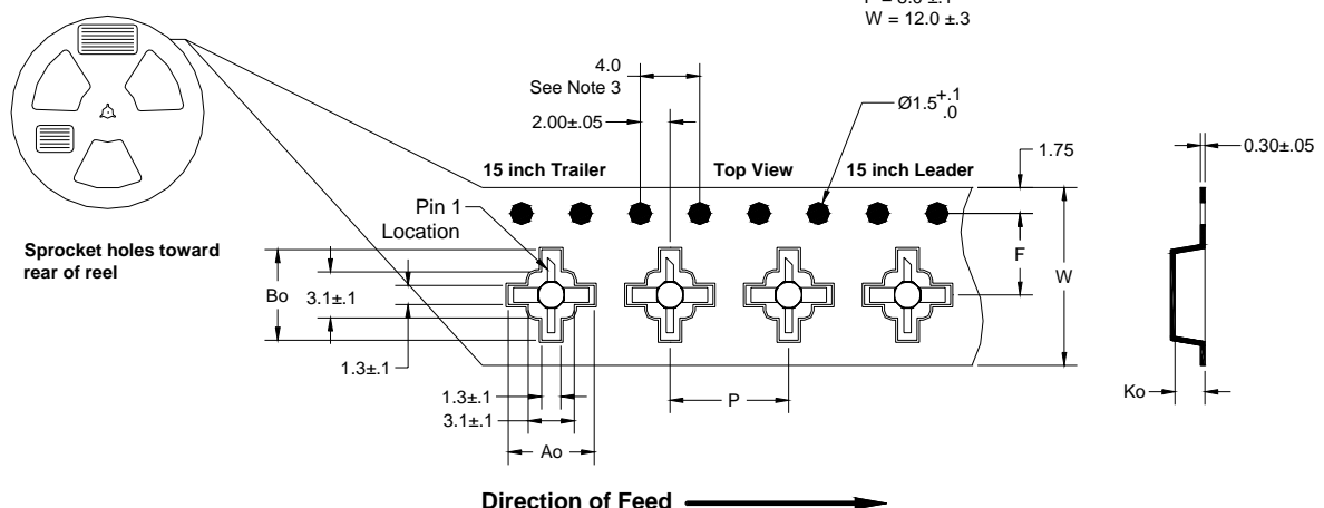
Figure 1. Carrier Tape Drawing with Part Orientation
