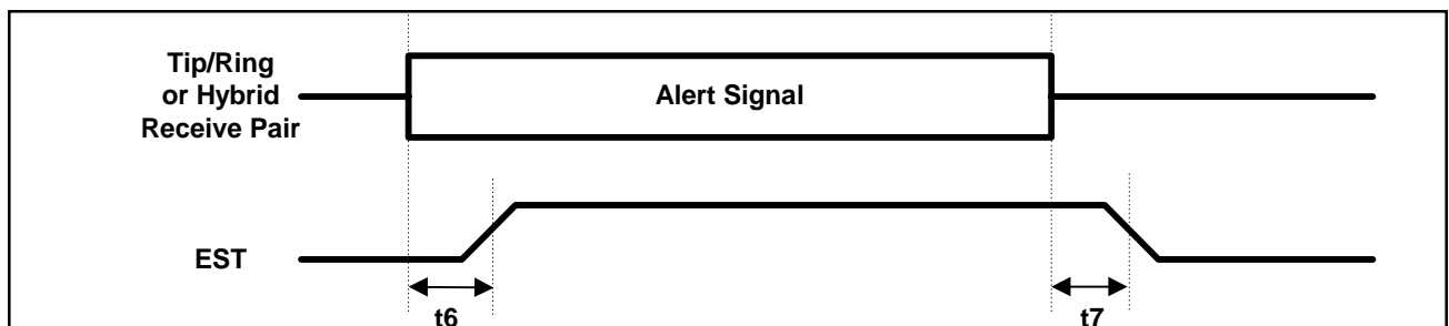
Figure-16. Dual Tone Alert Signal Detection Time
