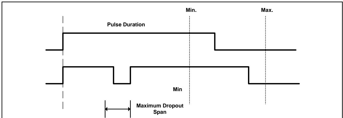
Figure-21. Valid DT-AS Pulses
