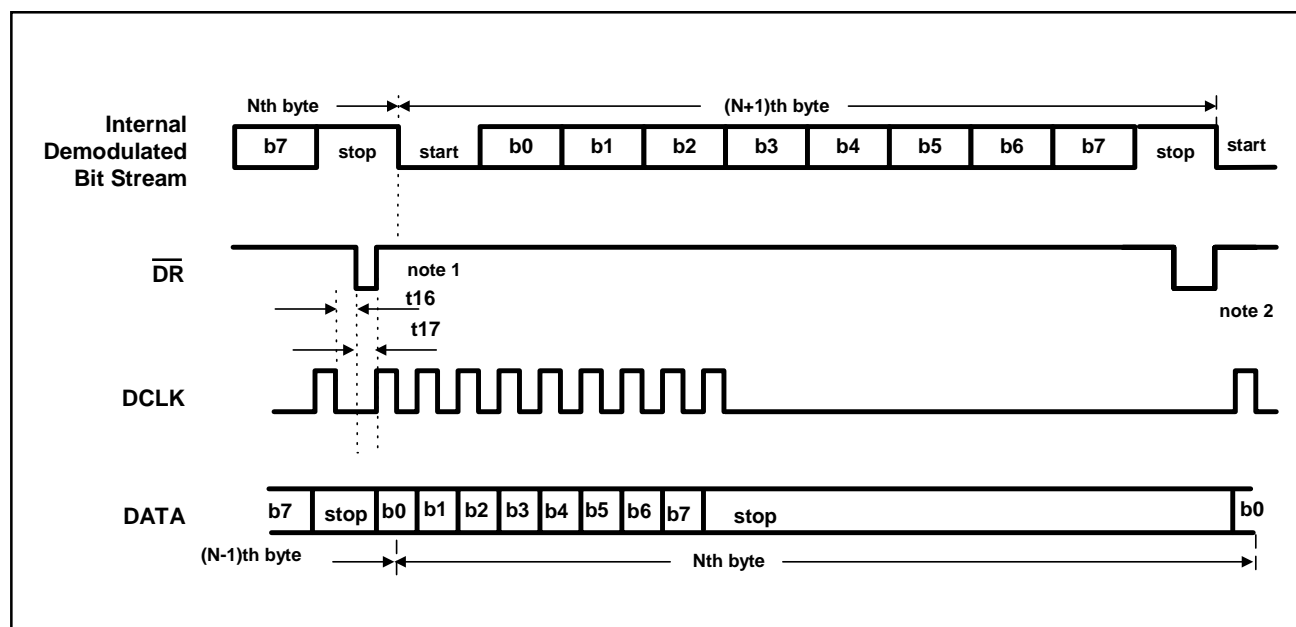
Figure-18. Serial Data Interface Timing in MODE '1'
