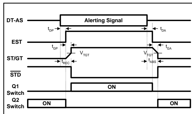
Figure-6. Guard Time Waveform
