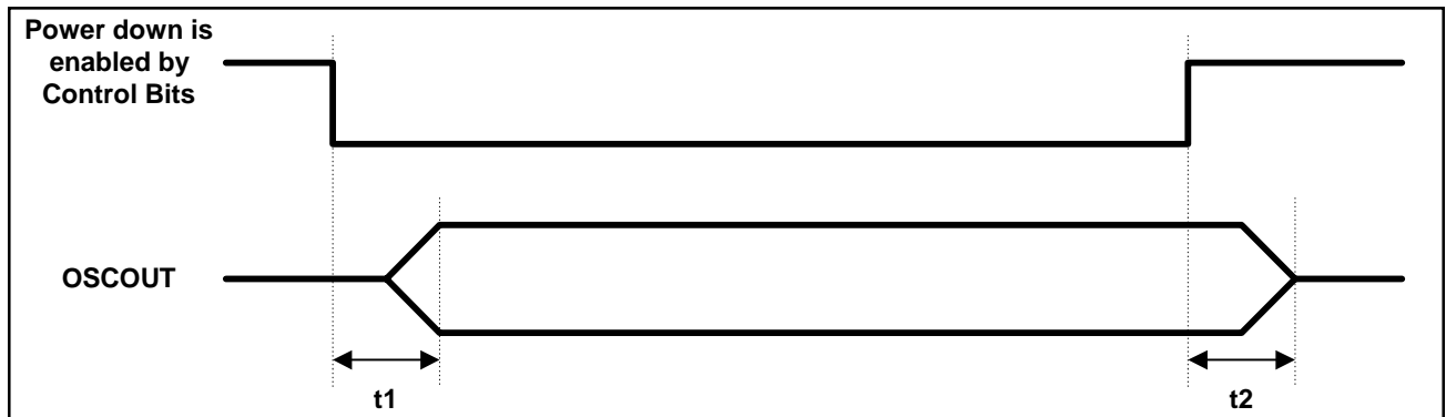
Figure-14. Power Up/Down Timing
