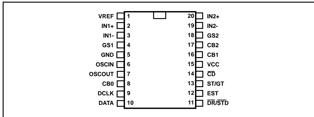
Figure-2. Pin Assignment
