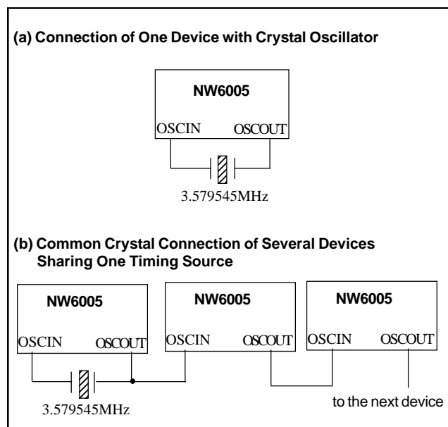
Figure-8. Application of Clock Driven Circuit
