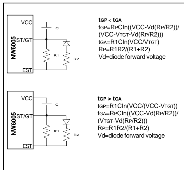
Figure-7. Guard Time Circuits with Unequal Present and Absent Times
