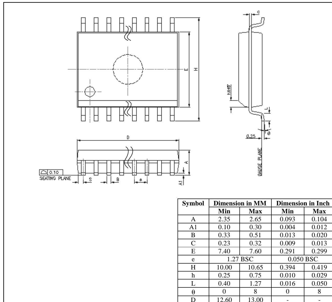
Figure-21. NW6005-XS 20 Pin SOIC Package Diagram
