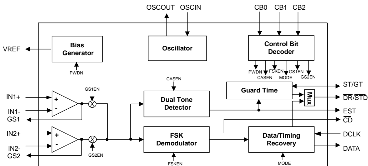
Figure-1. Block Diagram
