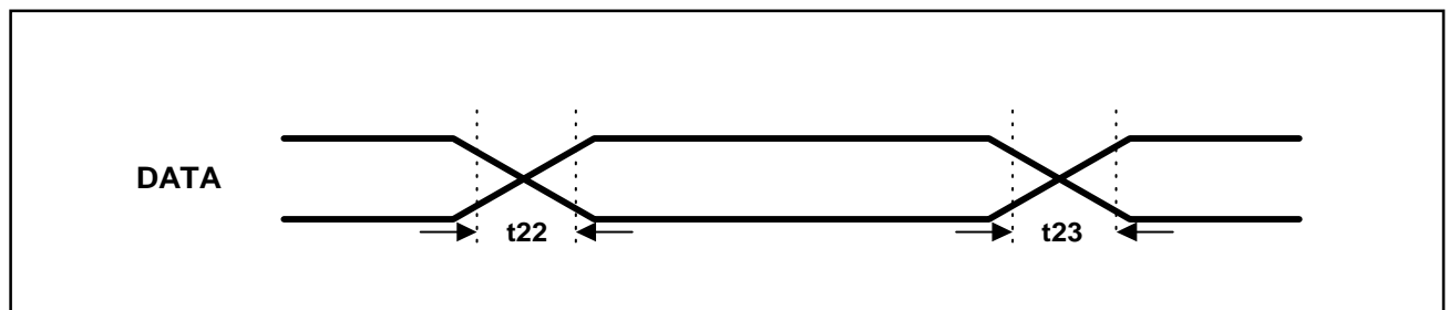
Figure-19. DATA Output Timing in Mode '0'
