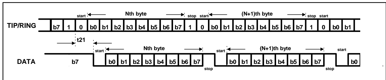
Figure-20. Serial Data Interface Timing in MODE '0'
