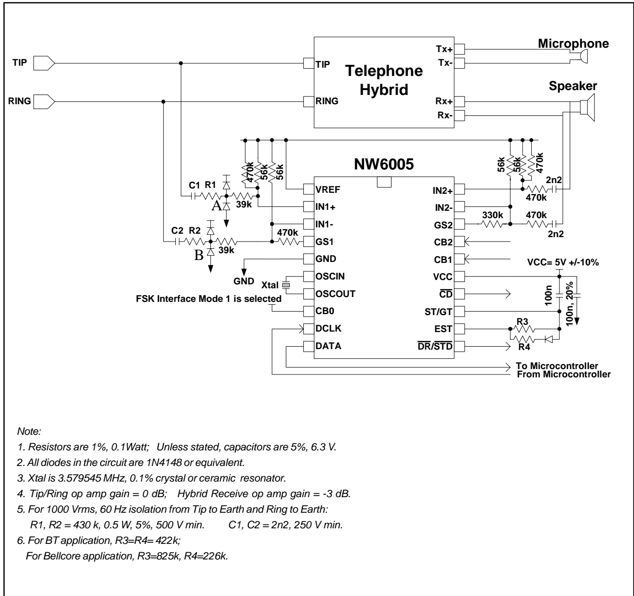
Figure-9. Typical Application Circuit For Bellcore MEI Compatible Type II Telephone, 5 V Operation
