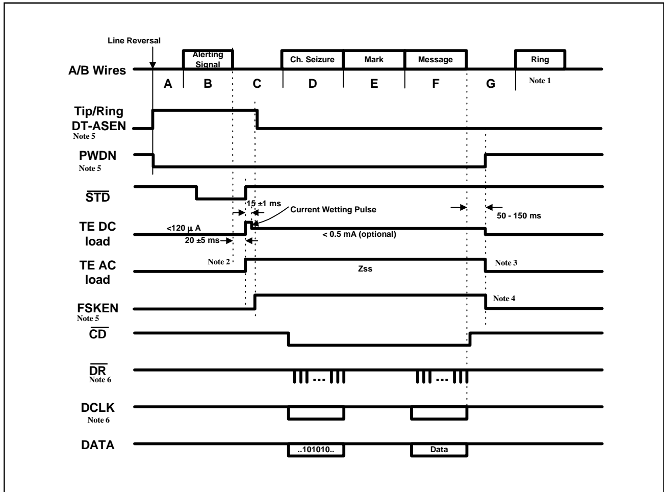
Figure-13. BT Idle State (on-hook) Data Transmission Timing Diagram
