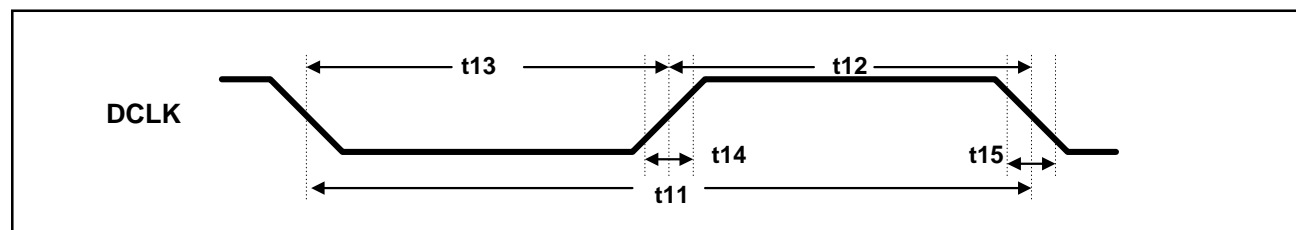
Figure-17. DCLK Timing in Mode '1'
