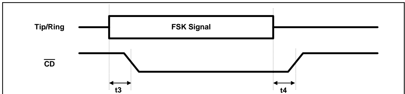
Figure-15. FSK Detection Time
