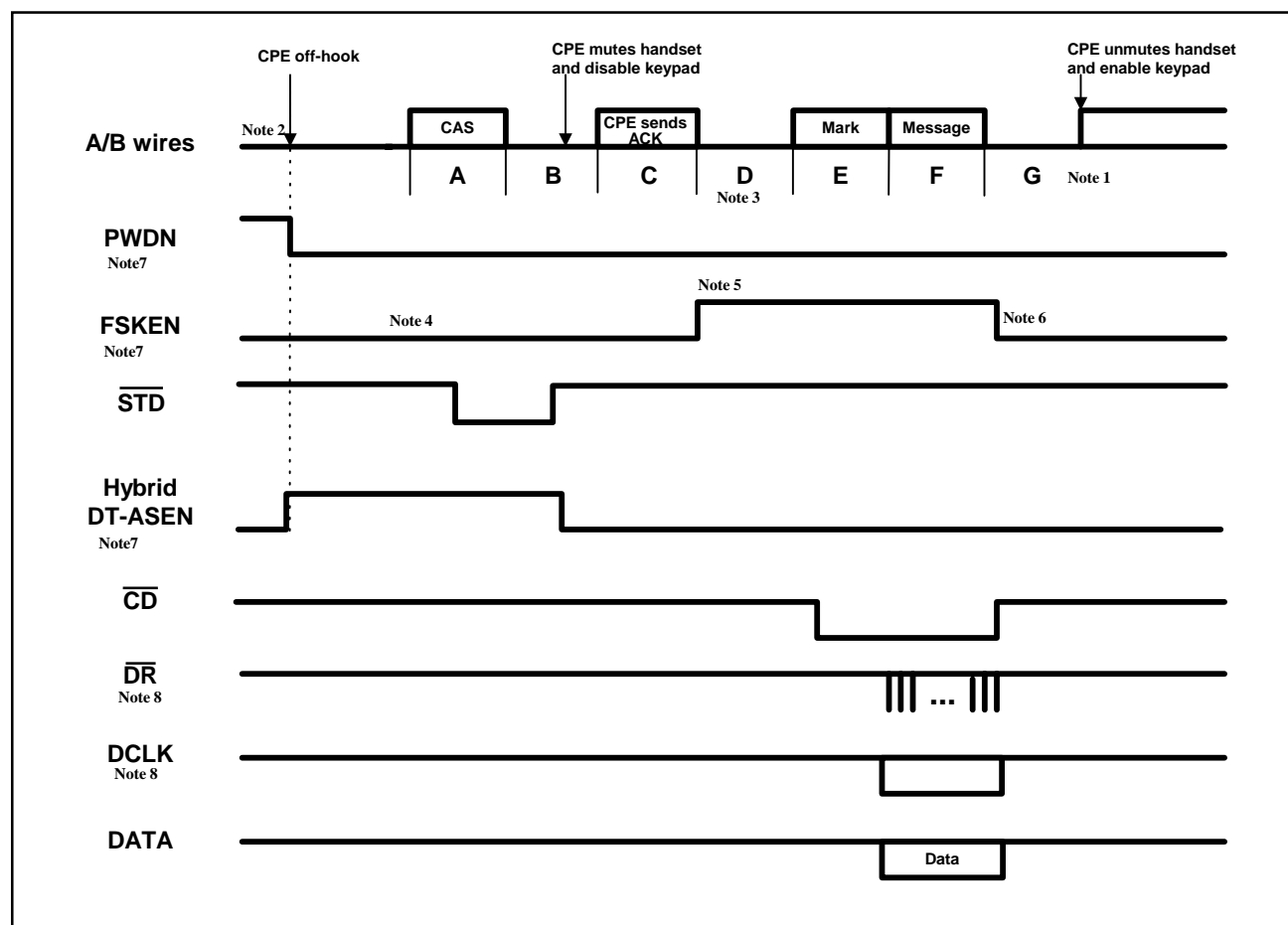
Figure-12. Bellcore Off-hook Data Transmission Timing Diagram
