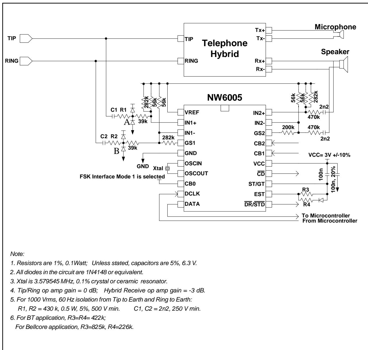
Figure-10. Typical Application Circuit For Bellcore MEI Compatible Type II Telephone, 3 V Operation
