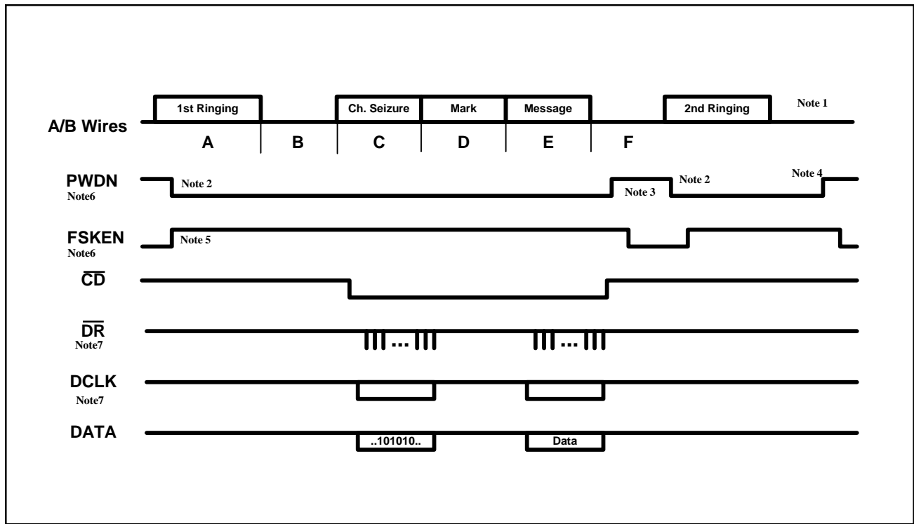
Figure-11. Bellcore On-hook Data Transmission Timing Diagram
