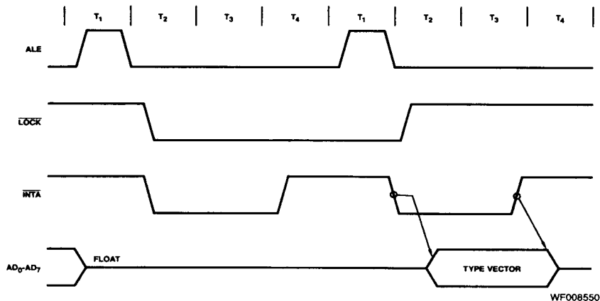
Figure 1. Interrupt Acknowledge Sequence
