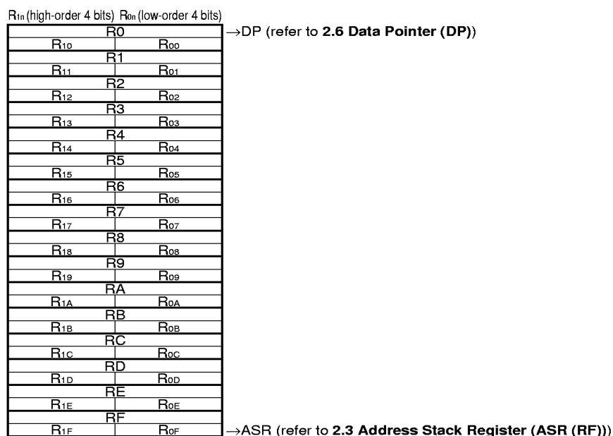
Figure 2-4. Data Memory Organization
