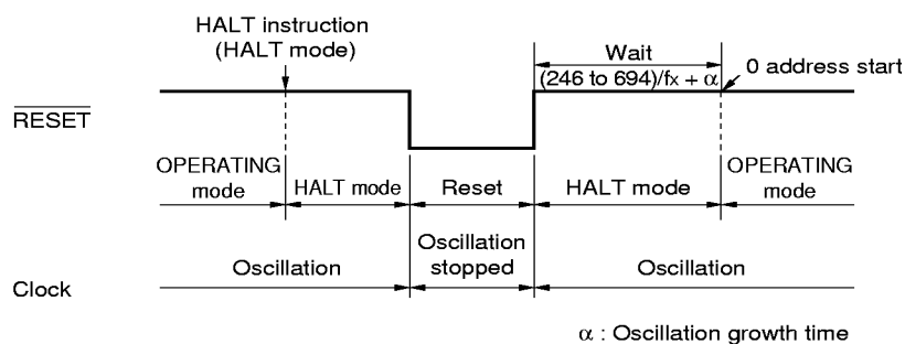
Figure 5-4. HALT Mode Release by \overline{\text{RESET}} Input
