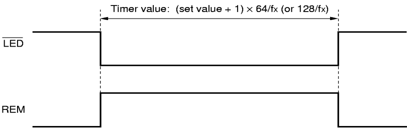
Figure 4-2. Timer Output (when carrier is not output)
