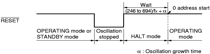
Figure 6-1. Reset Operation by RESET Input
