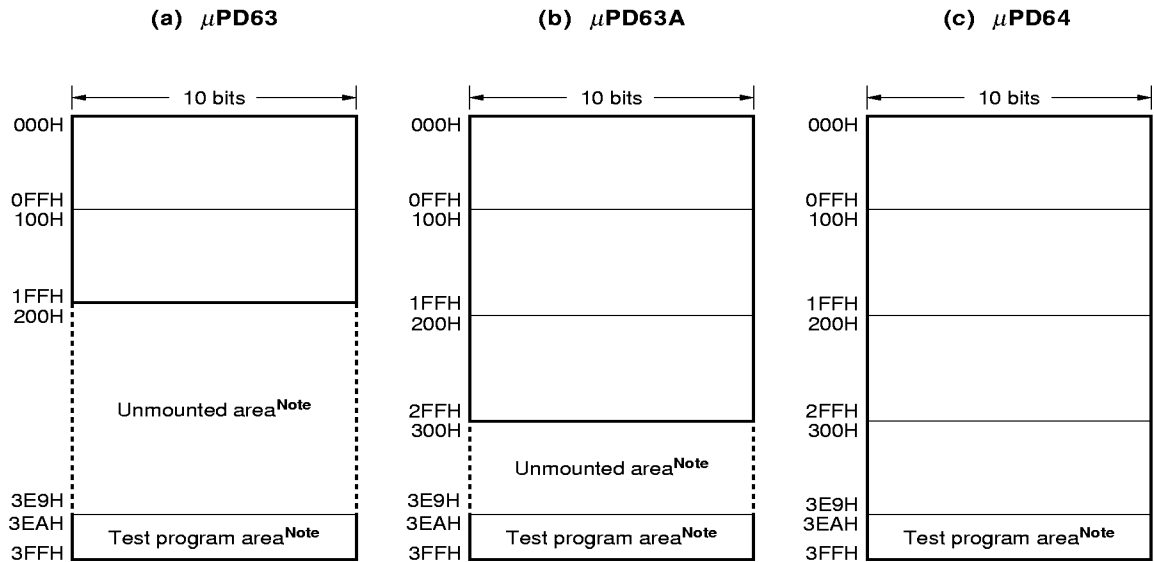
Figure 2-3. Program Memory Map
