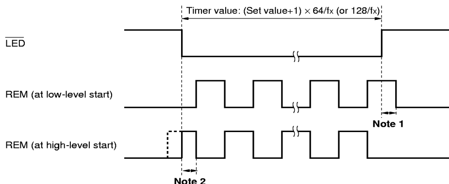
Figure 4-3. Timer Output (when carrier is output)
