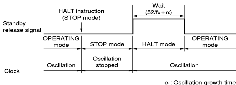
Figure 5-1. STOP Mode Cancellation by Release Condition
