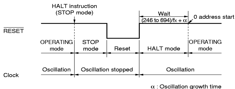
Figure 5-2. STOP Mode Release by \overline{\text{RESET}} Input
