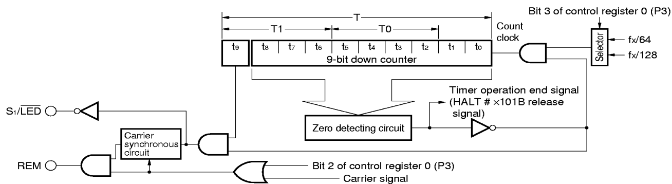
Figure 4-1. Timer Configuration
