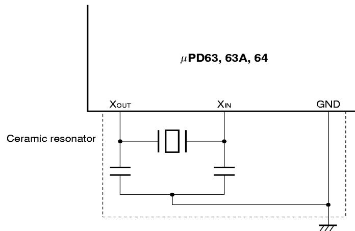
Figure 8-1. System Clock
