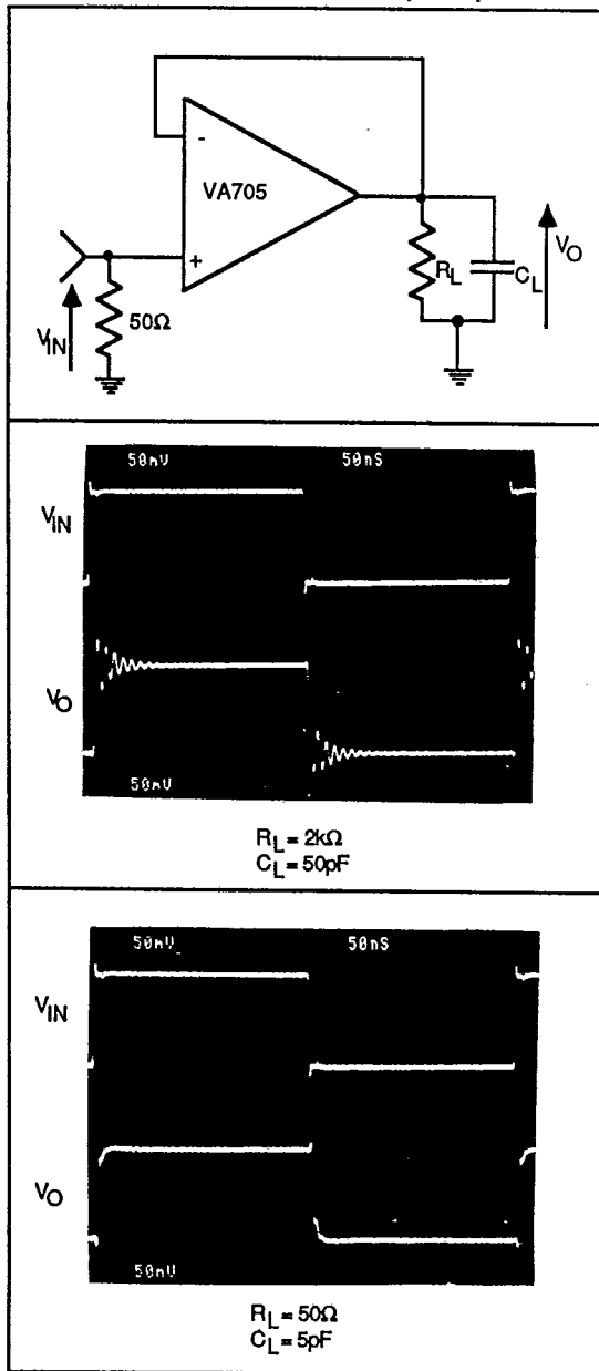
Figure 3: Unity Gain Follower Step Response
