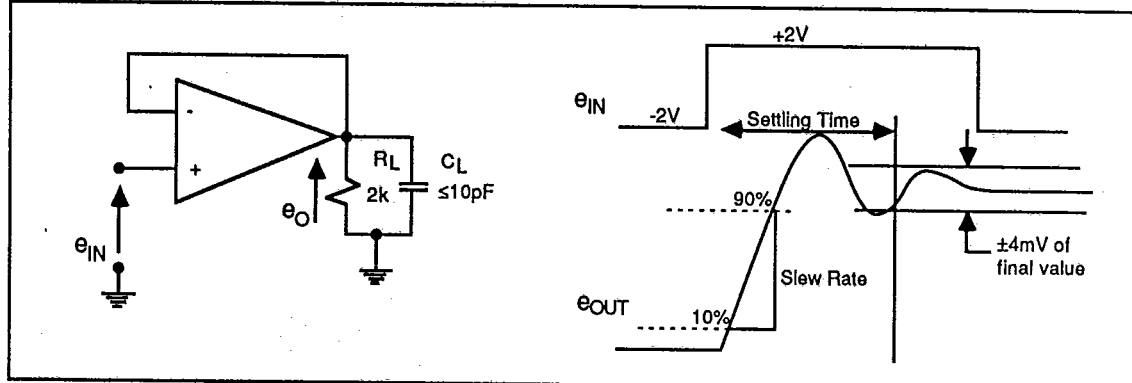
Figure 1b: Large Signal Response
