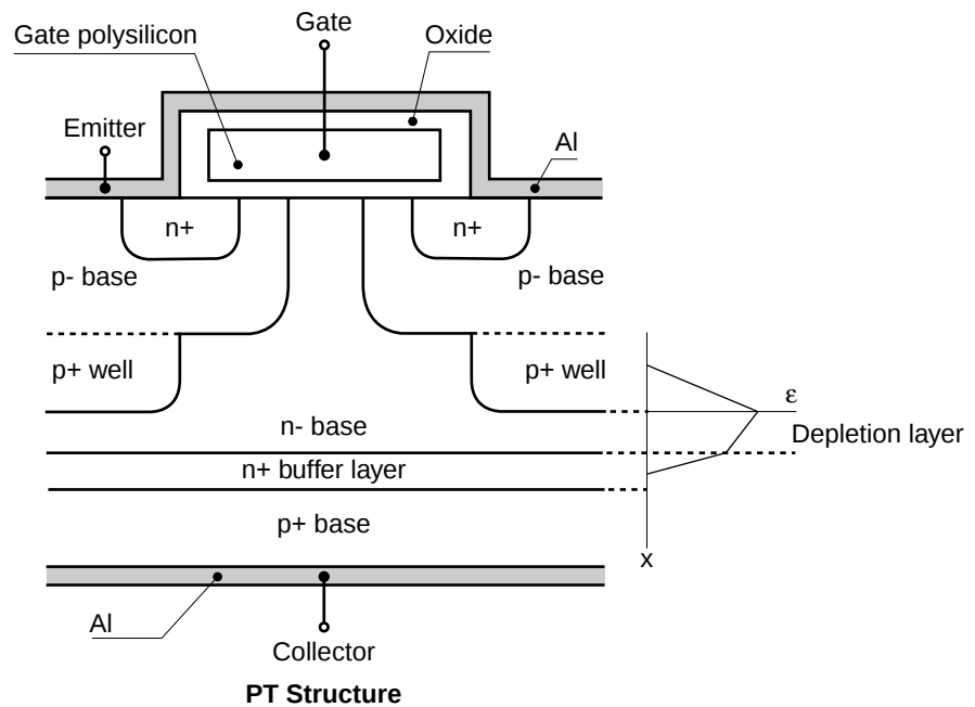
Fig.1 The structure of IGBTs
