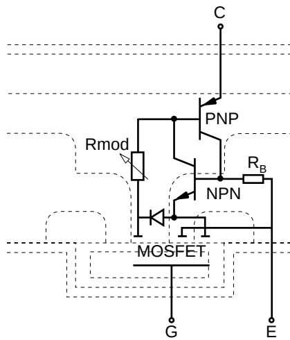
Fig.3a Equivalent circuit
