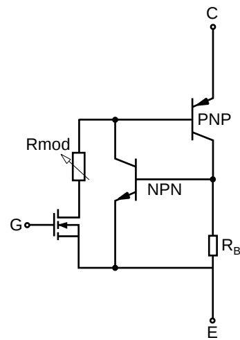
Fig.3b Equivalent circuit
