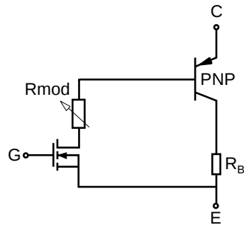
Fig.3c Equivalent circuit
