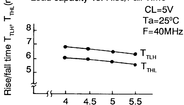
Load capacity vs. Rise/Fall Time
