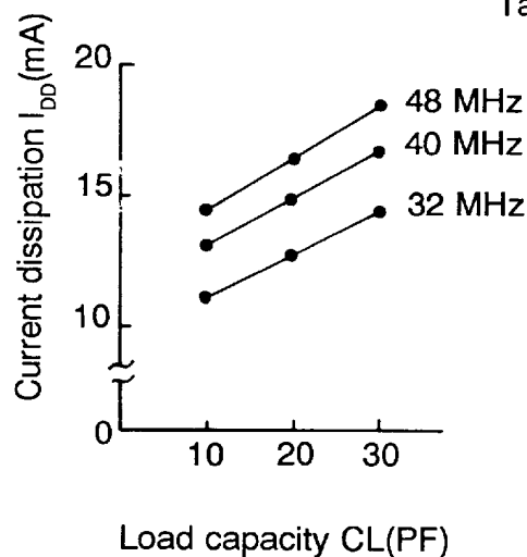
Current Dissipation vs. Load Capacity
