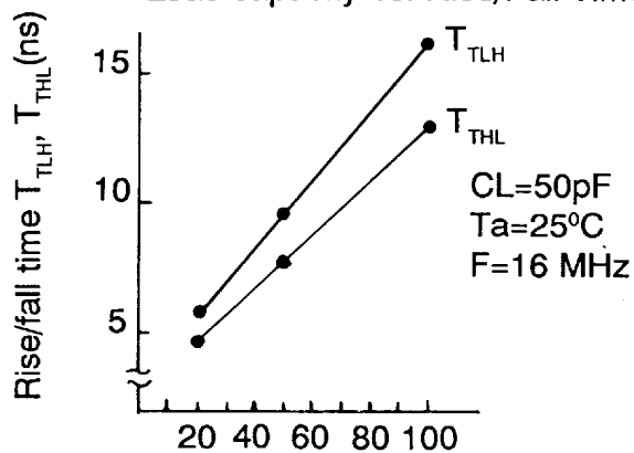
Load capacity vs. Rise/Fall Time
