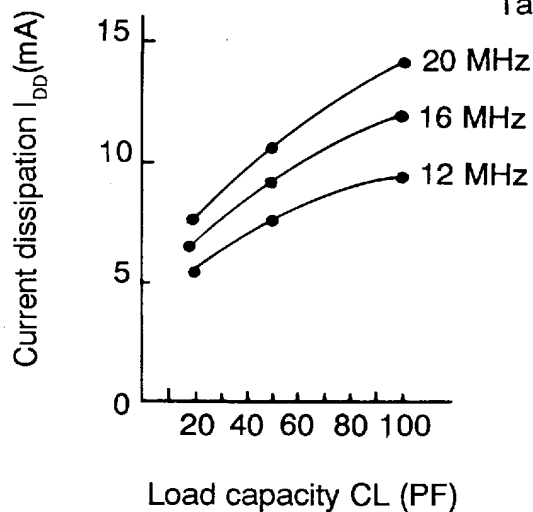
Current Dissipation vs. Load Capacity
