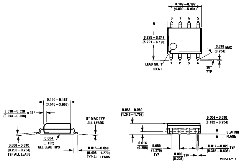
Molded Package SO (M) Order Number LM6261M or LM6361M NS Package Number M08A
