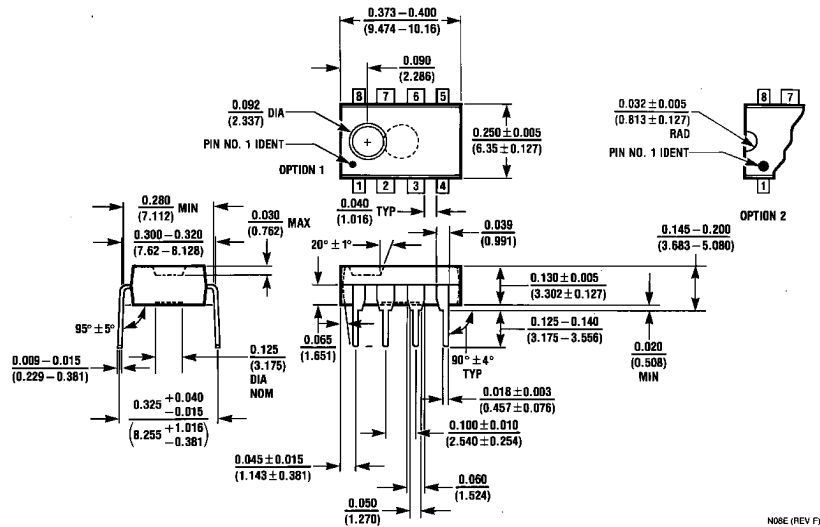
Molded Dual-In-Line Package (N) Order Number LM6261N or LM6361N NS Package Number NO8E
