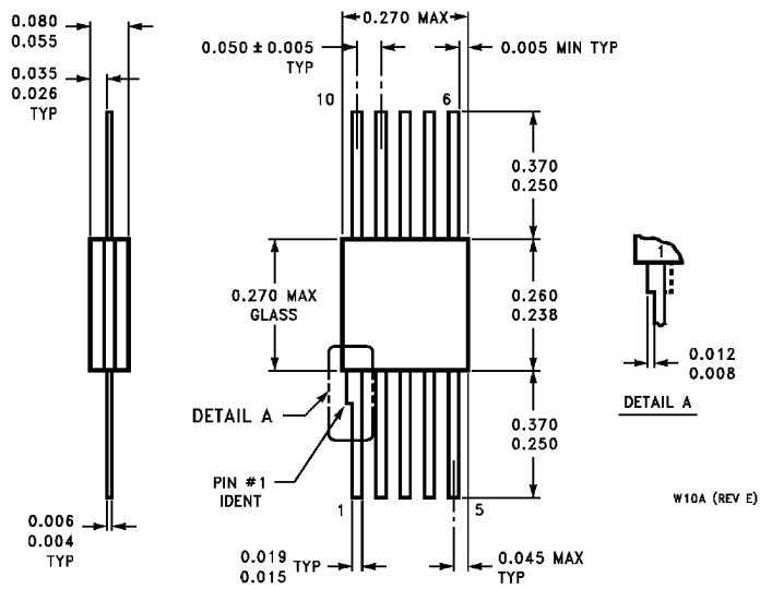
10-Pin Ceramic Flatpak Order Number LM6161W/883 NS Package Number W10A
