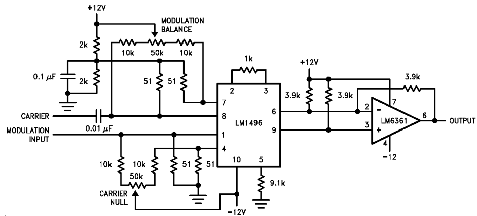
Modulator with Differential-to-Single-Ended Converter
