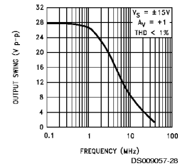
Power Bandwidth
