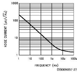
Input Noise Current
