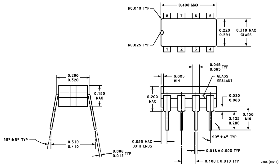
Ceramic Dual-In-Line Package (J) Order Number LM6161J/883 NS Package Number J08A
