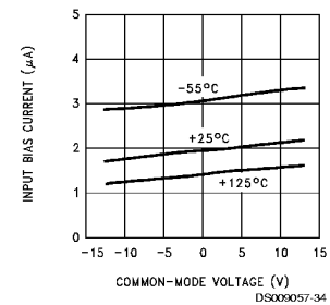
Bias Current vs Common-Mode Voltage
