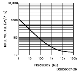
Input Noise Voltage
