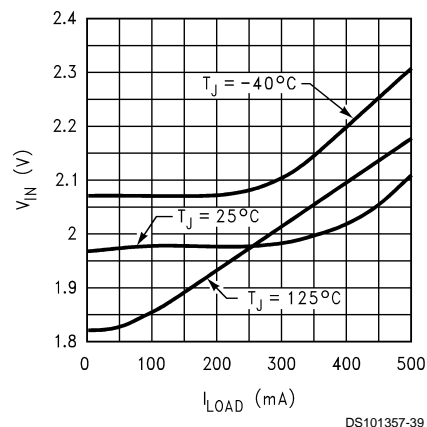
Minimum V_{IN} vs Load Current
