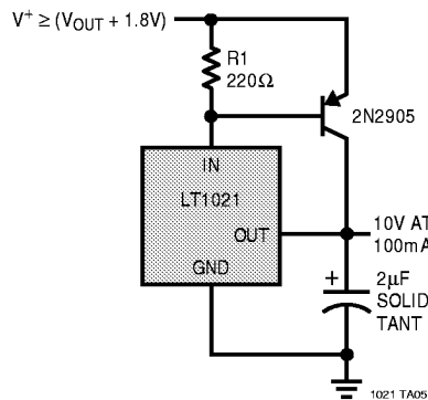
Boosted Output Current with No Current Limit
