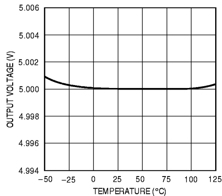
Output Voltage Temperature Drift LT1021-5
