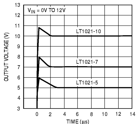
Start-Up (Series Mode)
