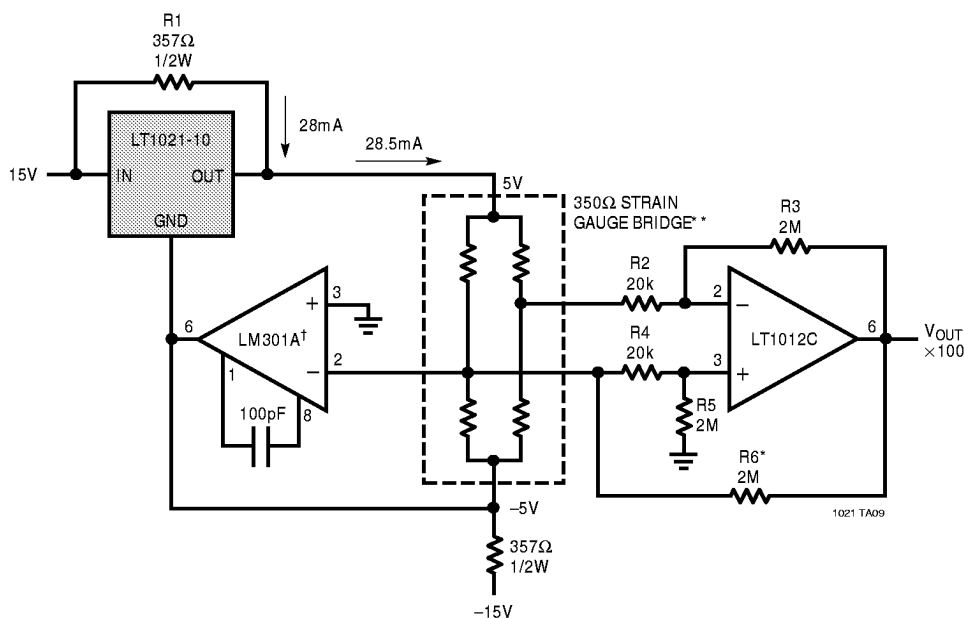
Strain Gauge Conditioner for 350Ω Bridge
