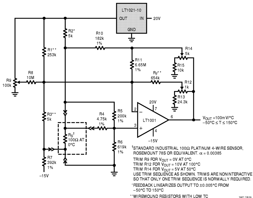
Ultralinear Platinum Temperature Sensor*
