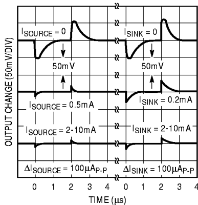
Load Transient Response LT1021-5, C_{LOAD} = 0
