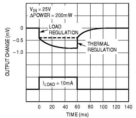
Thermal Regulation LT1021-5
