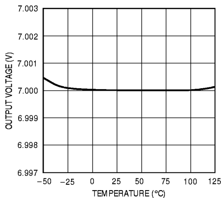
Output Voltage Temperature Drift LT1021-7
