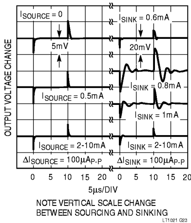
Load Regulation LT1021-7, LT1021-10
