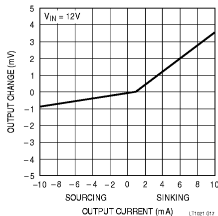
Load Regulation LT1021-7, LT1021-10
