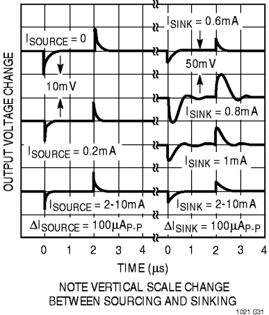
Load Transient Response LT1021-10, C LOAD = 0
