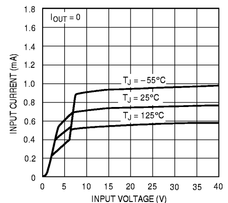
Quiescent Current LT1021-7
