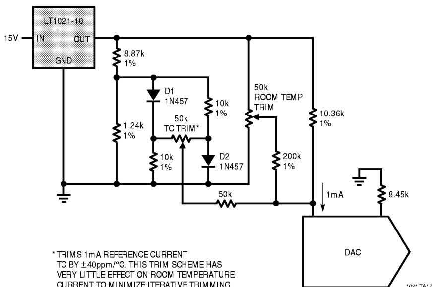
Precision DAC Reference with System TC Trim
