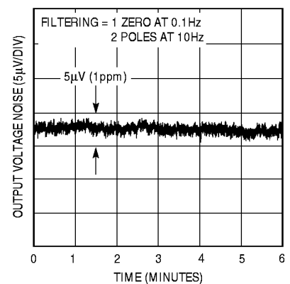
Output Noise 0.1Hz to 10Hz LT1021-5
