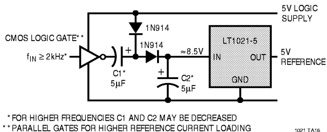
Operating 5V Reference from 5V Supply
