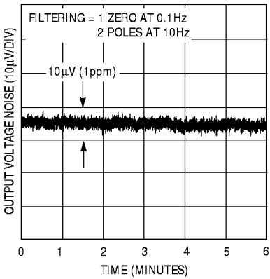
Output Noise 0.1Hz to 10Hz LT1021-10
