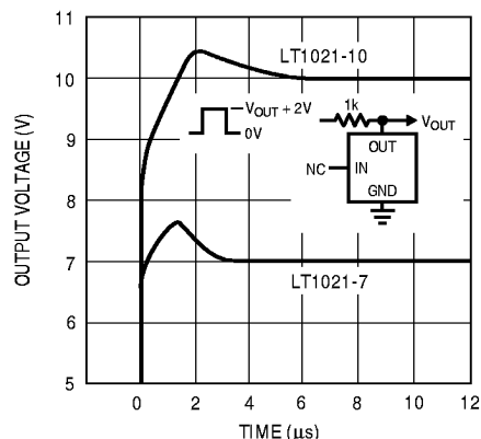
Start-Up (Shunt Mode) LT1021-7, LT1021-10
