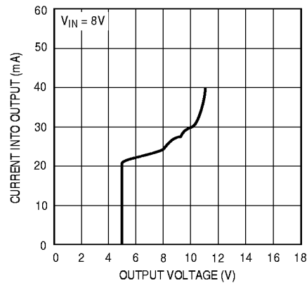
Sink Mode* Current Limit LT1021-5
