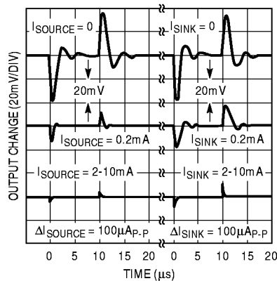
Load Transient Response LT1021-5, C_{LOAD} = 1000pF
