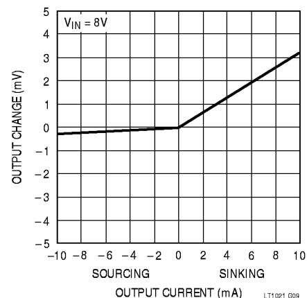
Load Regulation LT1021-5
