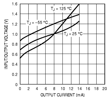
Minimum Input/Output Differential LT1021-7, LT1021-10
