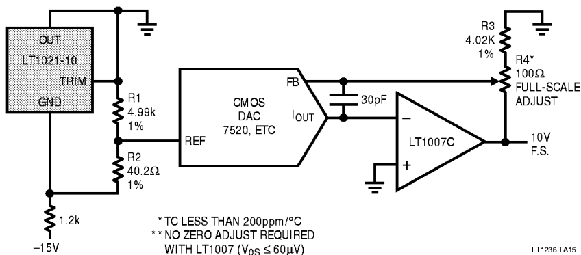
CMOS DAC with Low Drift Full-Scale Trimming**
