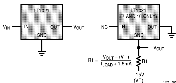
Basic Positive and Negative Connections
