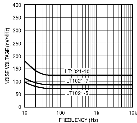
Output Voltage Noise Spectrum
