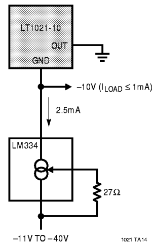
Negative Shunt Reference Driven by Current Source
