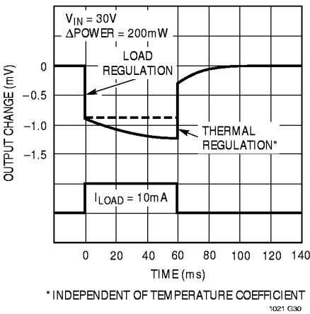
Thermal Regulation LT1021-10
