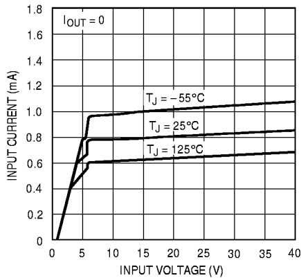
Quiescent Current LT1021-5
