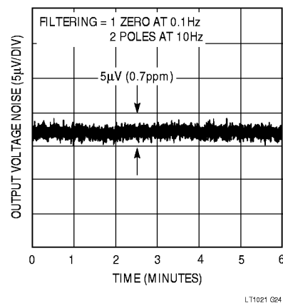
Output Noise 0.1Hz to 10Hz LT1021-7
