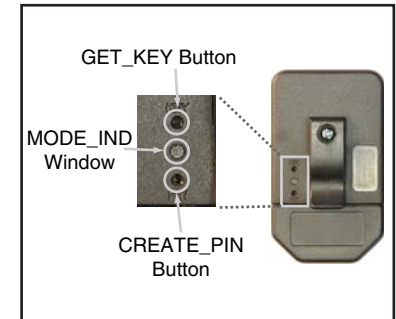
Figure 2: Button Access Holes
