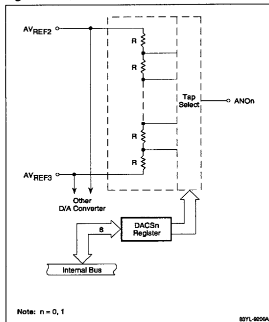
Figure 6. D/A Converter
