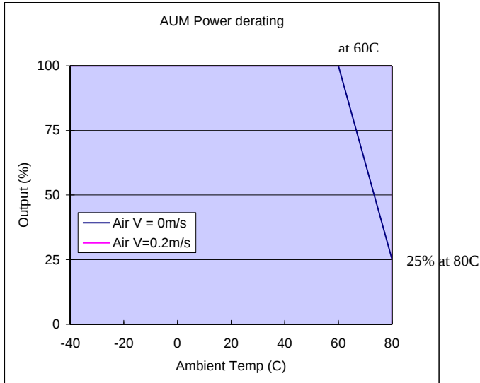
Derating Curve for the AUM Series
