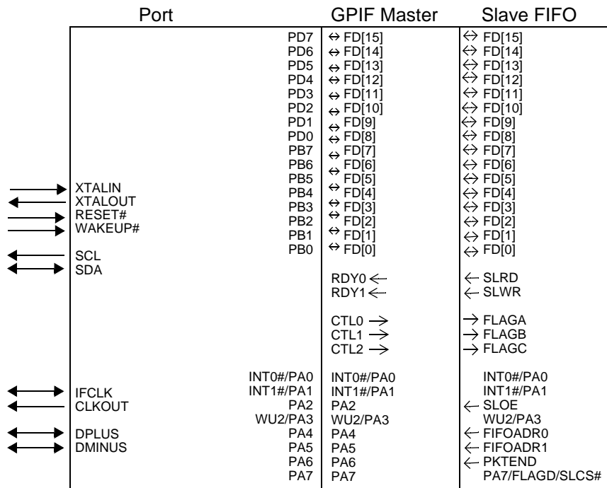
Figure 6. Signals
