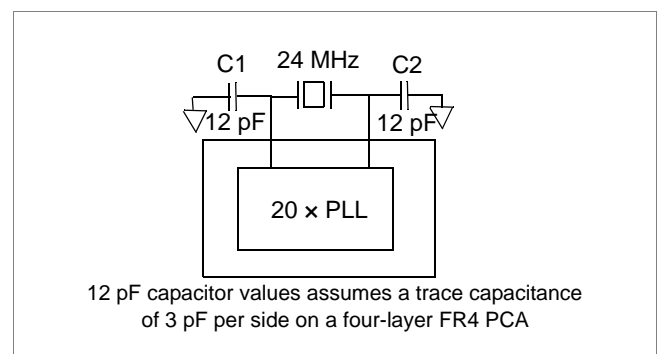
Figure 1. Crystal Configuration
