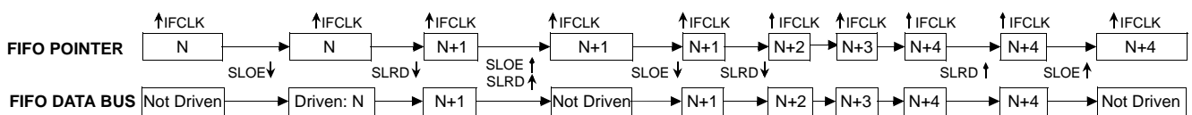
Figure 21. Slave FIFO Synchronous Sequence of Events Diagram
