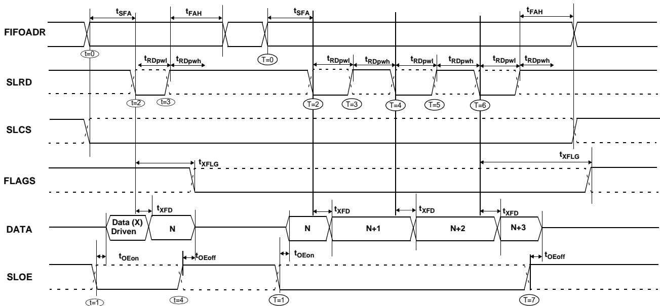
Figure 23. Slave FIFO Asynchronous Read Sequence and Timing Diagram [17]
