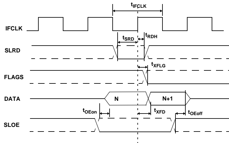
Figure 9. Slave FIFO Synchronous Read Timing Diagram [17]
