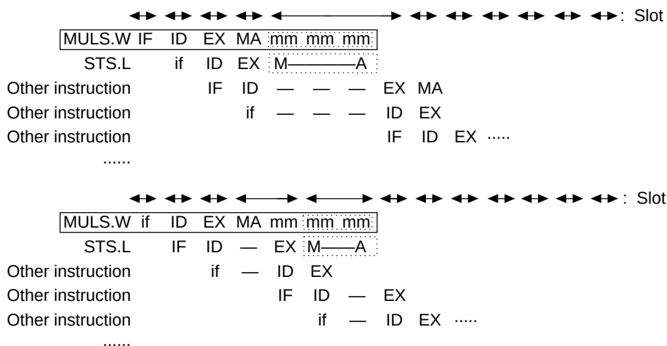
Figure 7.59 STS.L (Memory) Instruction Immediately After a MULS.W Instruction
