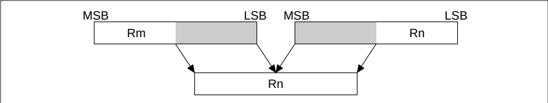
Figure 6.14 Extract
