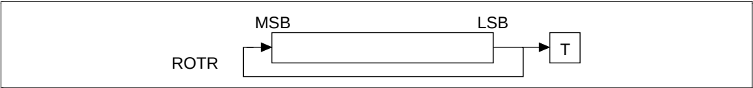
Figure 6.6 Rotate Right
