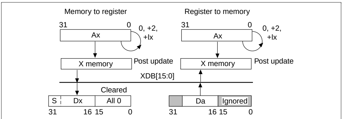
Figure 6.18 The MOVX Instruction
