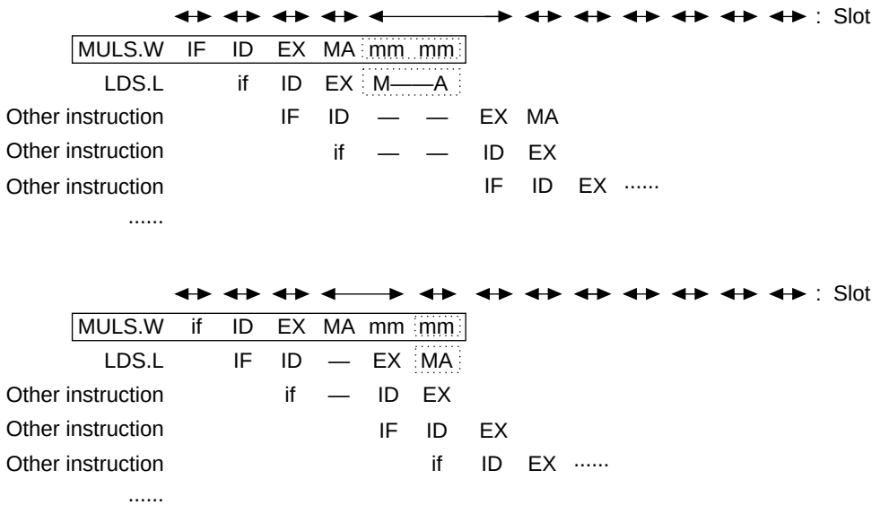
Figure 7.71 LDS.L (Memory) Instruction Immediately After a MULS.W Instruction
