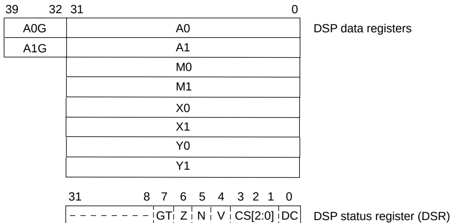
Figure 2.6 Organization of the DSP Registers
