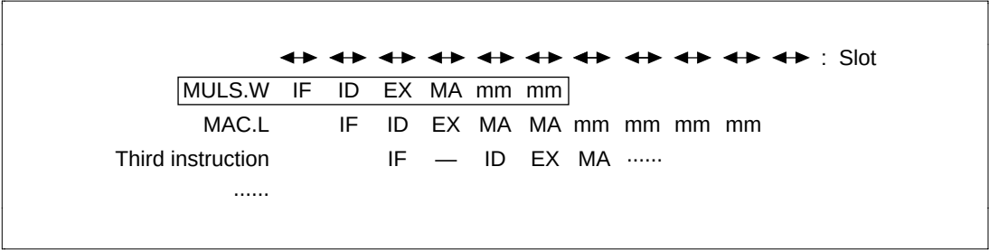
Figure 7.64 MAC.L Instruction Immediately After a MULS.W Instruction
