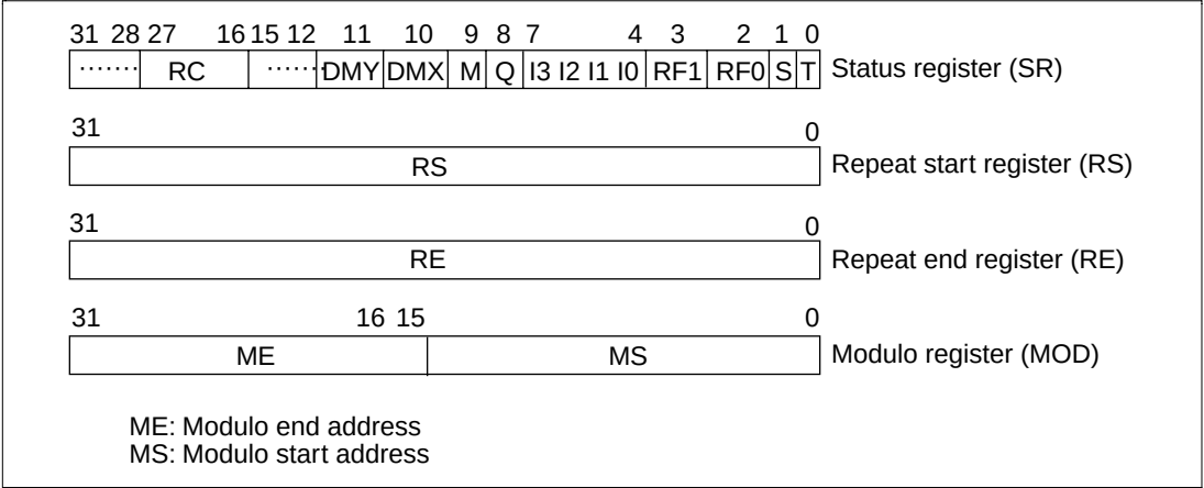
Figure 2.4 Organization of the Control Registers (SH-DSP)
