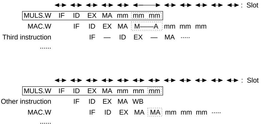
Figure 7.55 MAC.W Instruction Immediately After a MULS.W Instruction
