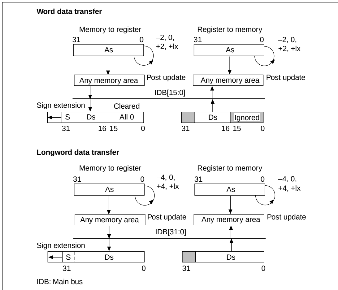
Figure 6.17 The MOVSW Instruction
