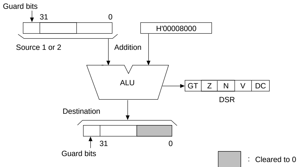
Figure 4.17 Rounding Flowchart
