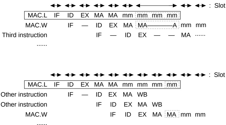
Figure 7.47 MAC.W Instruction Immediately After a MAC.L Instruction
