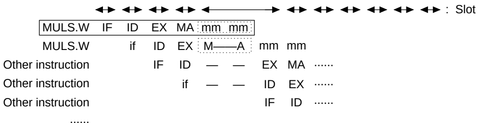
Figure 7.66 MULS.W Instruction Immediately After Another MULS.W Instruction (IF and MA contention)
