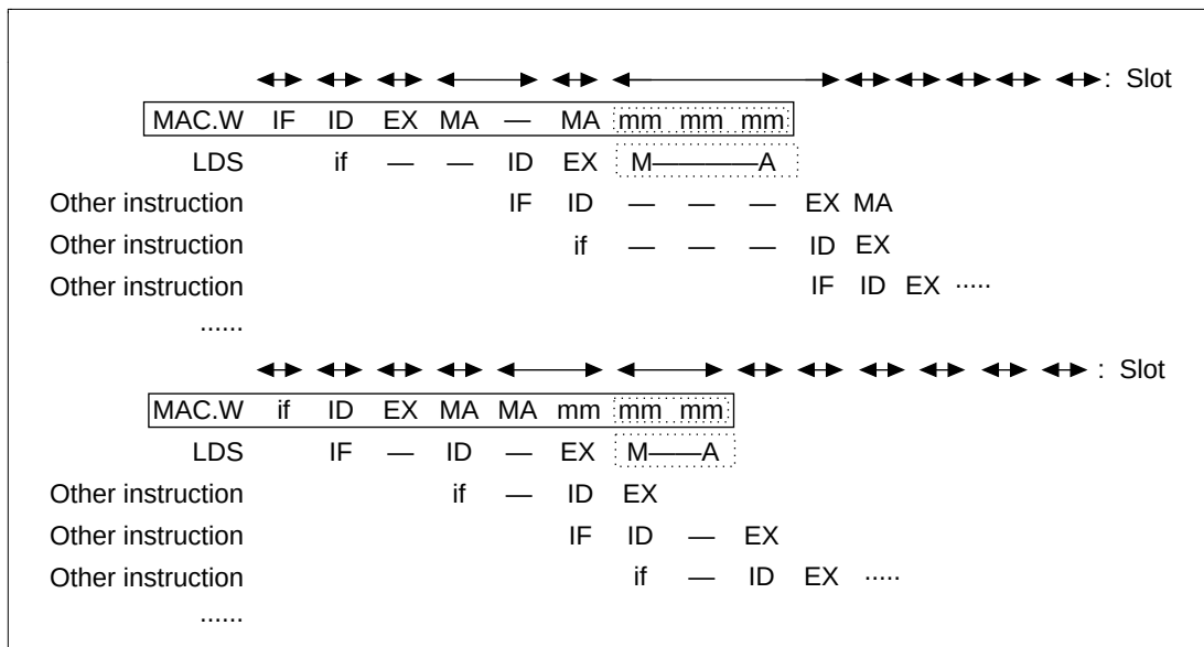
Figure 7.30 LDS (Register) Instruction Immediately After a MAC.W Instruction
