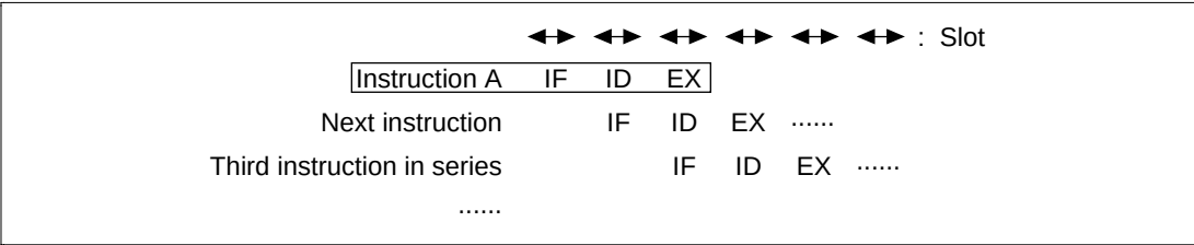
Figure 7.74 Register-Register Logic Operation Instruction Pipeline
