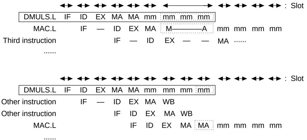
Figure 7.73 MAC.L Instruction Immediately After a DMULS.L Instruction
