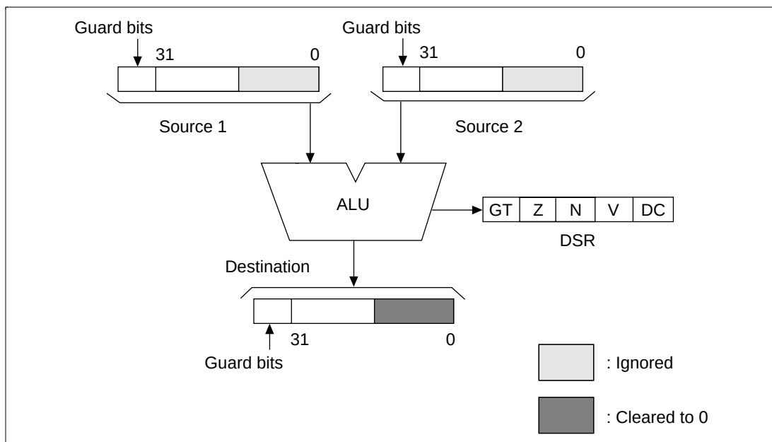
Figure 4.11 ALU Integer Operation Flowchart
