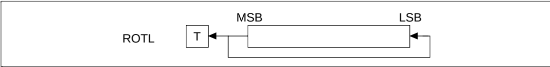
Figure 6.5 Rotate Left
