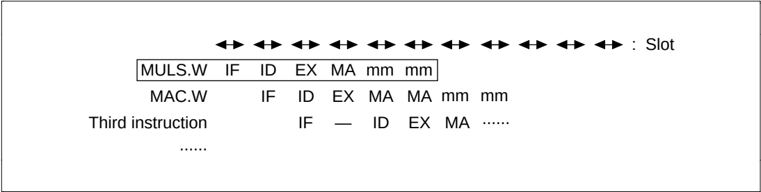
Figure 7.63 MAC.W Instruction Immediately After a MULS.W Instruction
