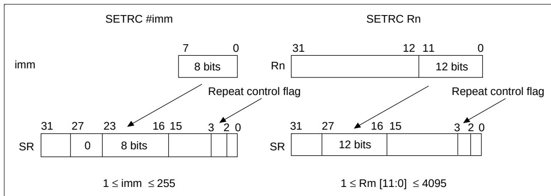
Figure 6.7 SETRC Instruction
