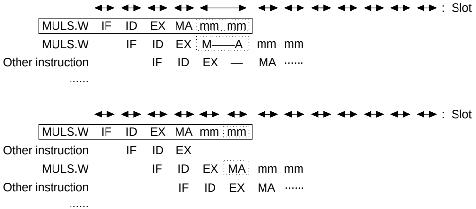
Figure 7.65 MULS.W Instruction Immediately After Another MULS.W Instruction
