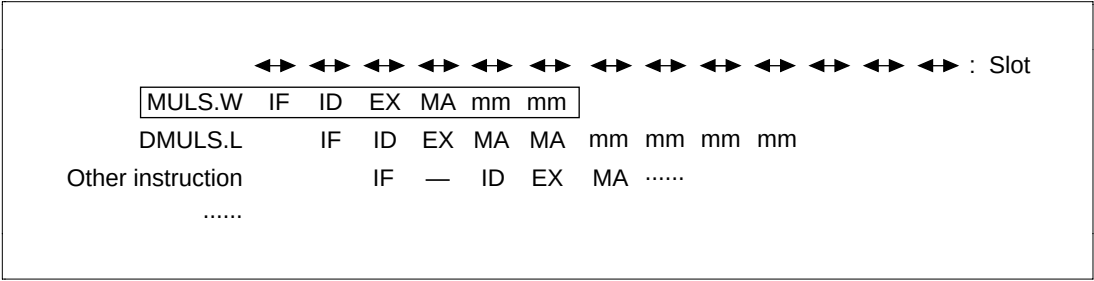
Figure 7.67 DMULS.L Instruction Immediately After a MULS.W Instruction
