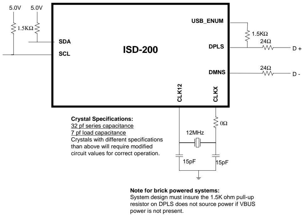
Figure 6 – External Components Connection
