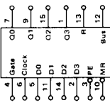
MC4316/4016 MC4318/4018
