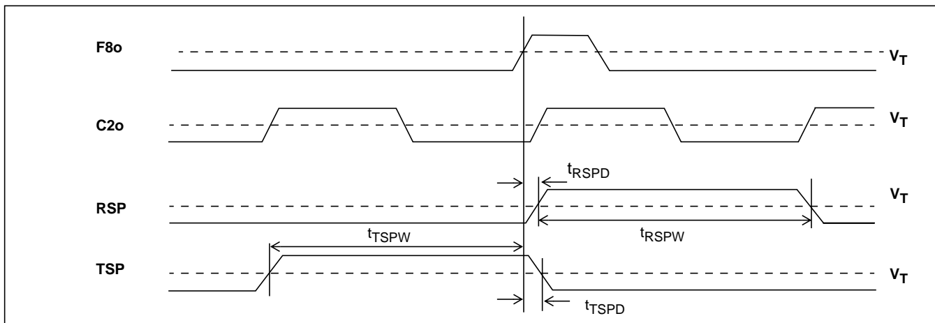
Figure 14 - Output Timing 2
