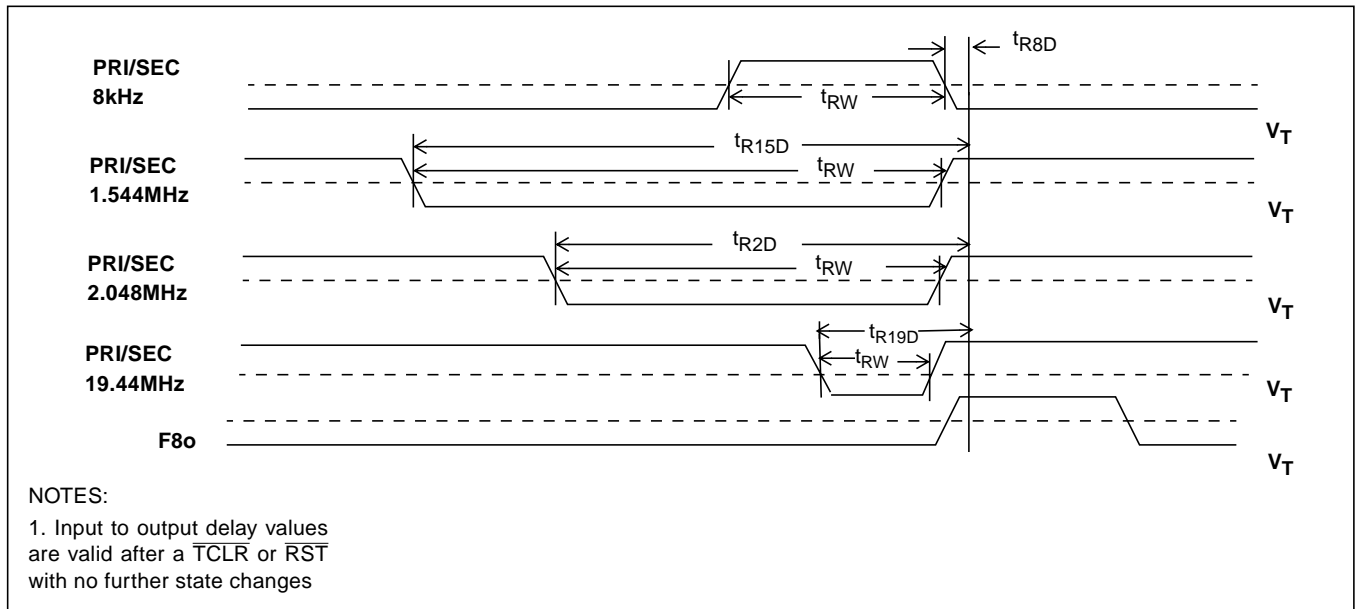
Figure 12 - Input to Output Timing (Normal Mode)
