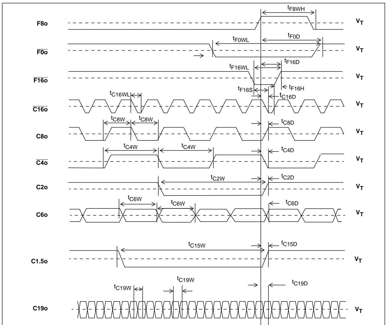
Figure 13 - Output Timing 1
