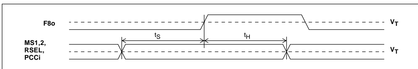
Figure 15 - Input Controls Setup and Hold Timing
