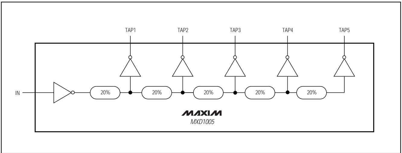
Functional Diagram
