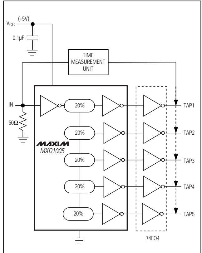
Figure 2. Test Circuit
