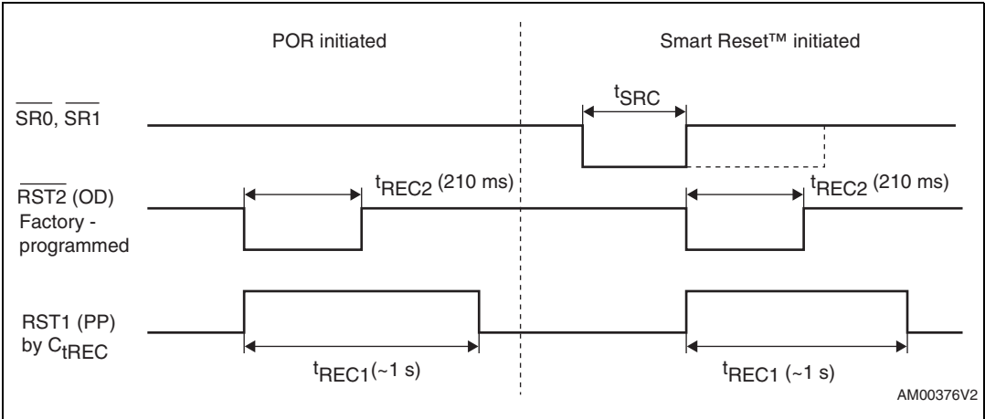
Figure 5. Timing waveforms
