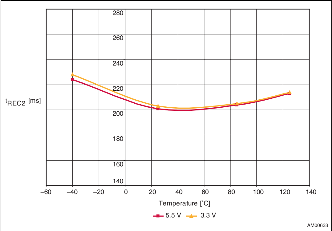
Figure 7. Output reset timeout period t_{REC2} vs. temperature and supply voltage V_{CC} ( t_{REC} option E)
