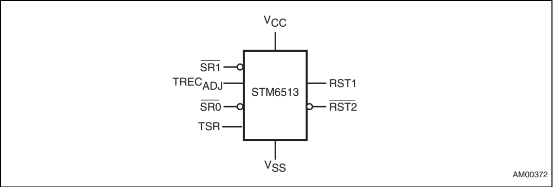
Figure 1. Logic diagram
