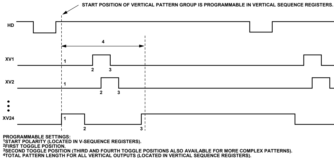
Figure 35. Vertical Pattern Group Programmability
