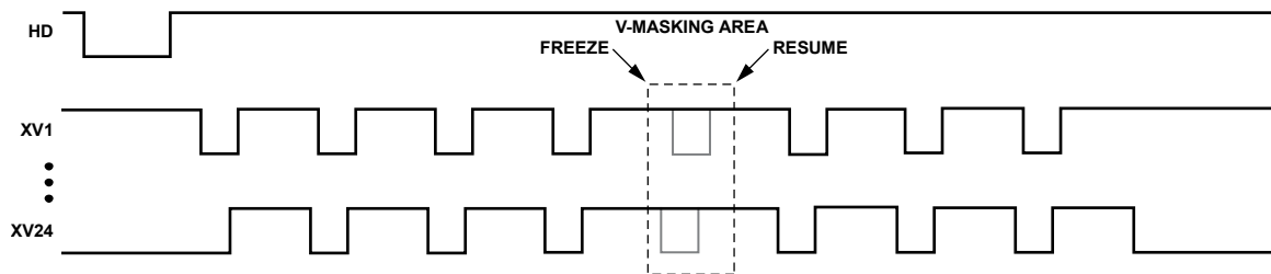
Figure 45. Using FREEZE/RESUME
