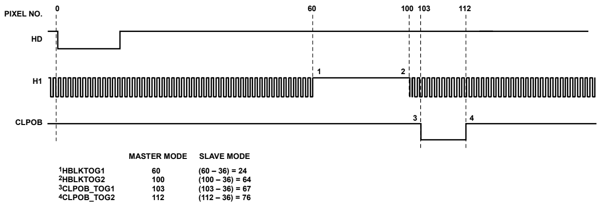
Figure 90. Example of Slave Mode Register Setting to Obtain Desired Toggle Positions
