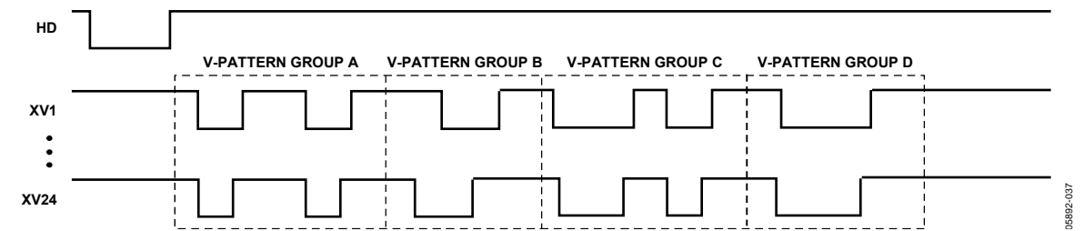
Figure 38. Combining Multiple V-Patterns Using CONCAT_GRP = 1
