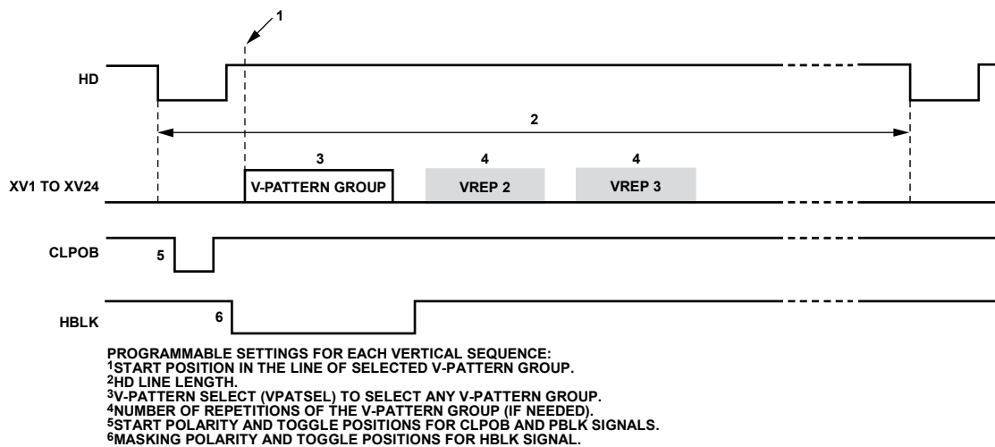
Figure 36. V-Sequence Programmability
