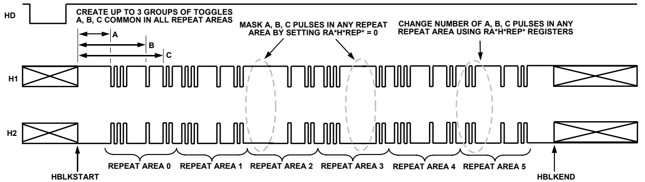
Figure 30. HBLK Mode 2 Operation
