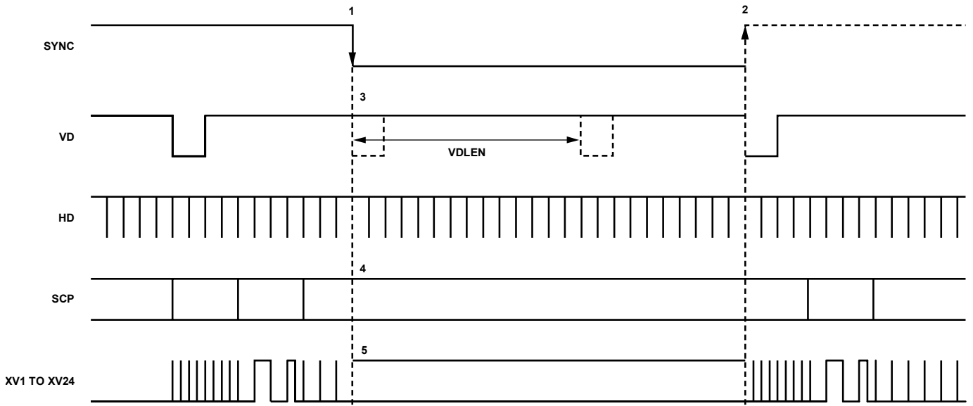
Figure 79. Default Mode 1
