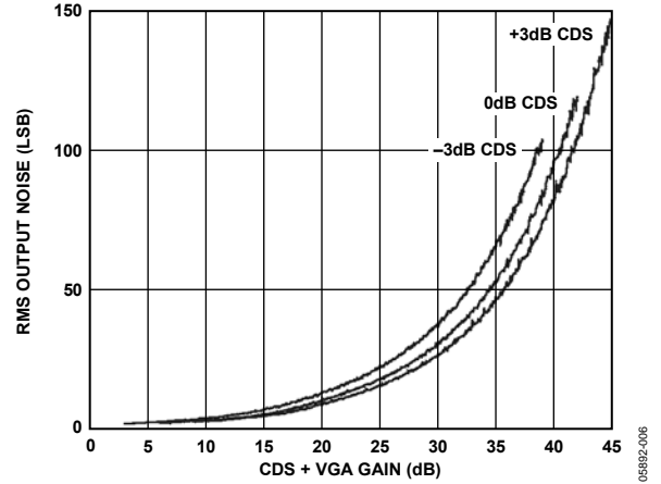
Figure 6. Output Noise vs. Total Gain (CDS + VGA)
