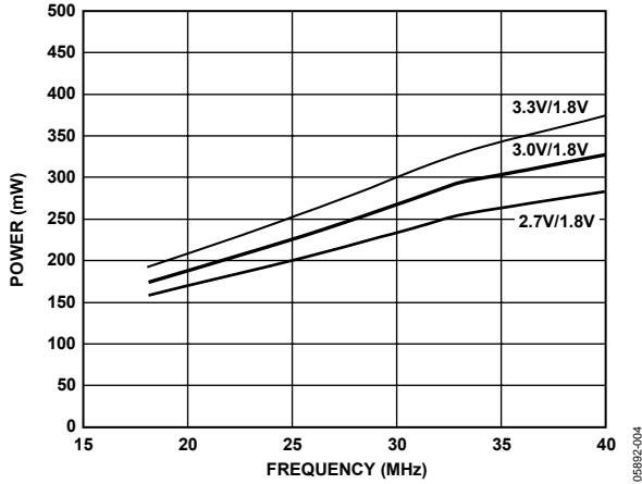
Figure 4. AFETG Power vs. Frequency (V-Driver not Included) (AVDD = TCVDD = DVDD = 1.8 V, All Other Supplies at 2.7 V, 3.0 V, or 3.3 V)
