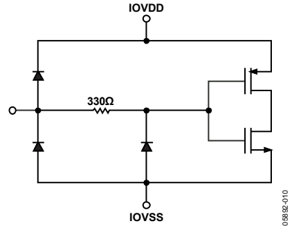
Figure 10. Digital Inputs
