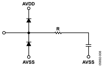
Figure 8. CCDIN
