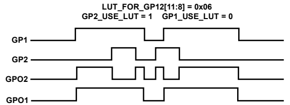
Figure 77. LUT Example for GP1 XOR GP2
