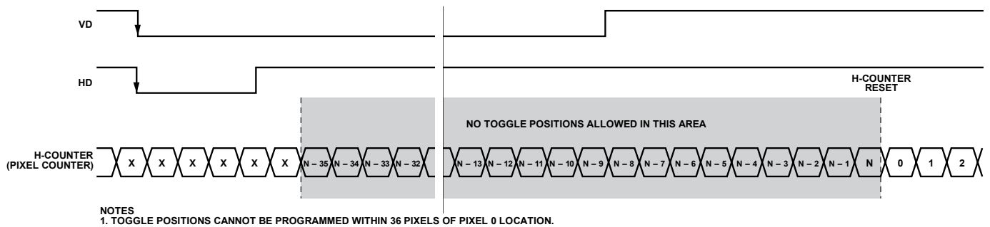
Figure 92. Toggle Position Inhibited Area—Slave Mode
