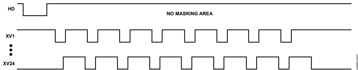
Figure 44. No FREEZE/RESUME
