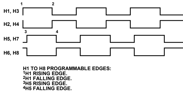
Figure 19. HCLK Mode 3 Operation
