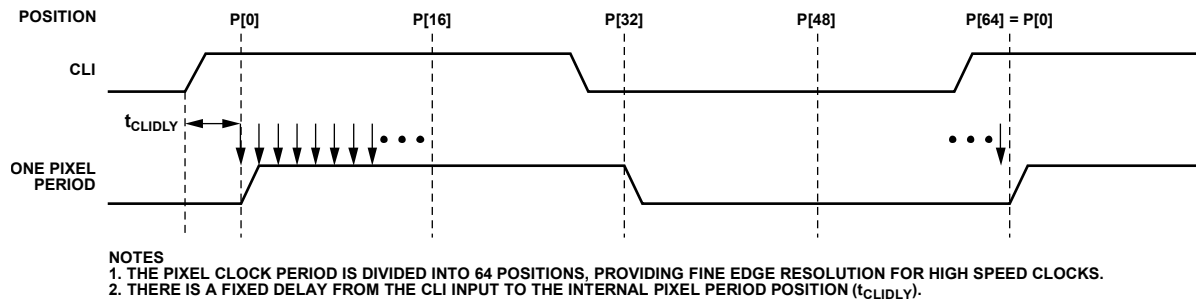
Figure 16. High Speed Clock Resolution from CLI, Master Clock Input
