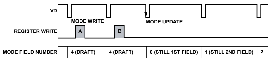
Figure 65. Update of MODE Register, SCK Updated (Default Setting)
