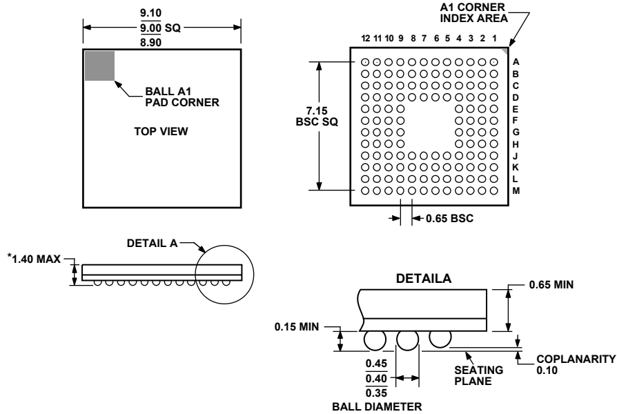
Figure 102. 128-Lead Chip Scale Package Ball Grid Array [CSP_BGA] 9 mm × 9 mm Body (BC-128) Dimensions shown in millimeters
