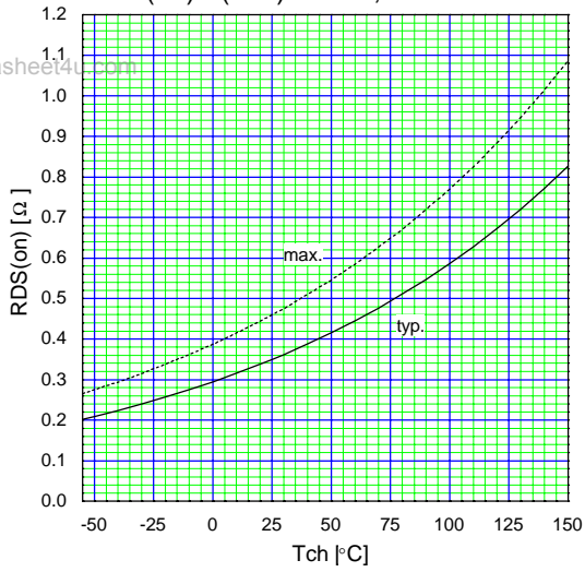
Drain-Source On-state Resistance R_{DS(on)}=f(T_{ch}):I_D=7A, V_{GS}=10V
