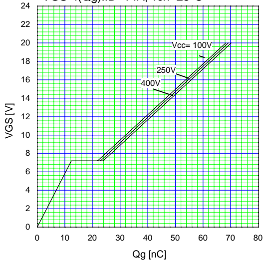
Typical Gate Charge Characteristics V_{GS}=f(Q_g):I_D=14A, T_{ch}=25^{\circ}C
