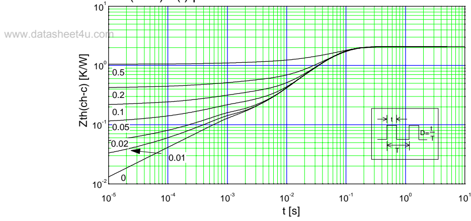
Transient Thermal impedance Z_{th}(ch-c)=f(t) parameter: D=t/T
