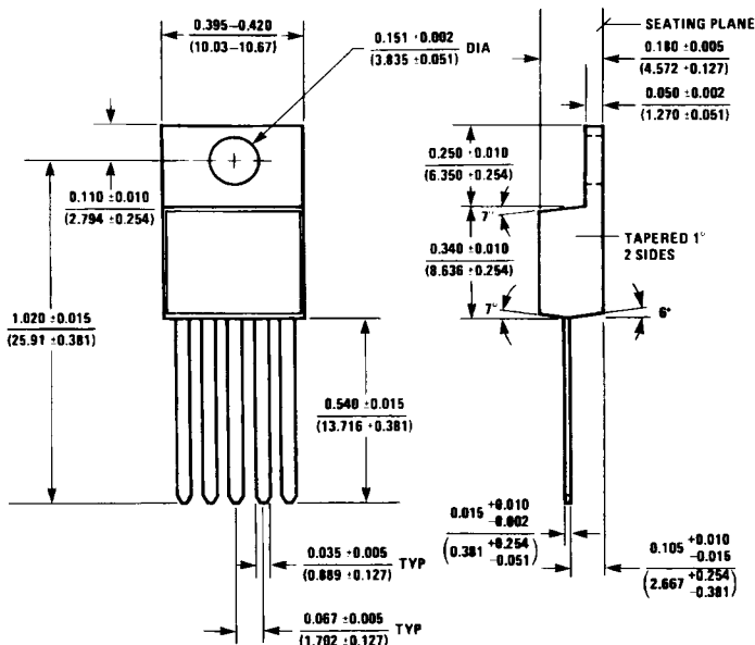
5-Lead TO-220 (T) Order Number LM2576T-ADJ NS Package Number T05A
