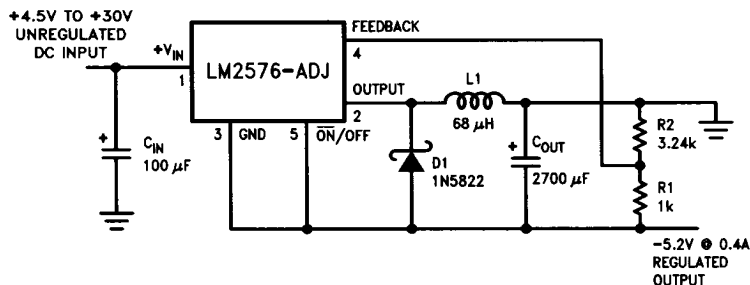
FIGURE 6. Inverting Buck-Boost
