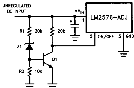
FIGURE 7. Undervoltage Lockout
