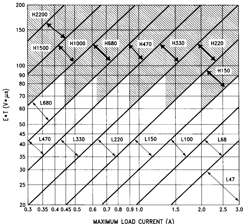
FIGURE 4. Inductor Value Selection Guide (for Continuous Mode Operation)
