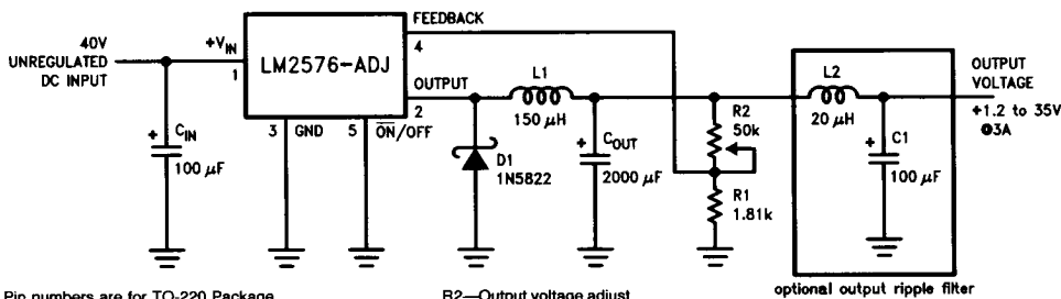
FIGURE 8. 1.2V to 35V Adjustable 3A Power Supply with Low Output Ripple
