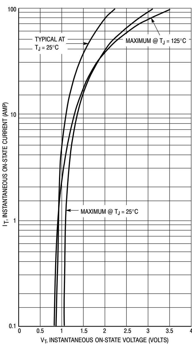
Figure 3. On-State Characteristics
