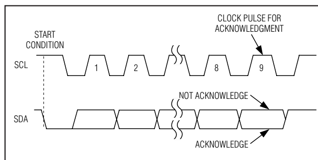
Figure 7. Acknowledge
