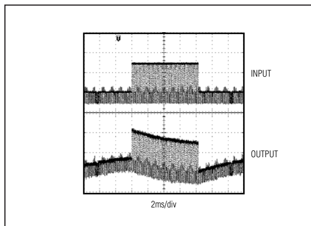
Figure 4. AC-Coupled Output
