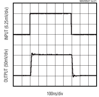
SMALL-SIGNAL PULSE RESPONSE (FLTEN = 0)
