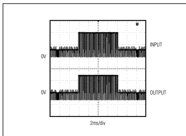
Figure 5. DirectDrive Output
