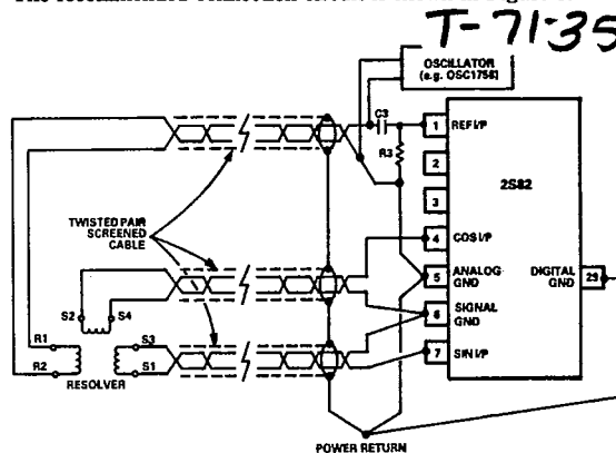
Figure 8. Connecting the 2S82 to a Resolver
