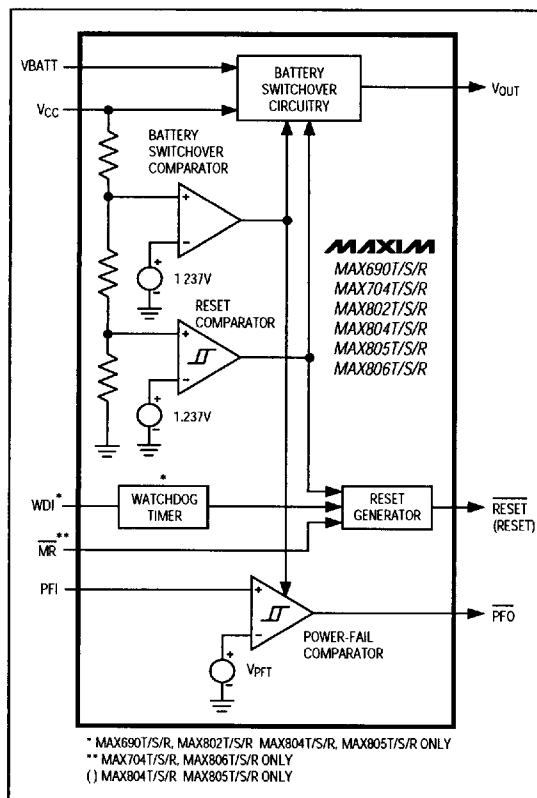
Figure 1. Block Diagram
