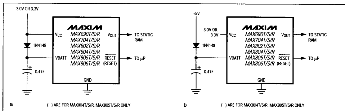
Figure 3. Using a SuperCap as a Backup Power Source
