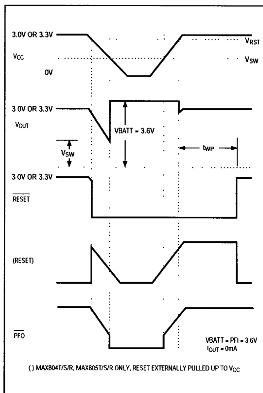
Figure 2. Timing Diagram
