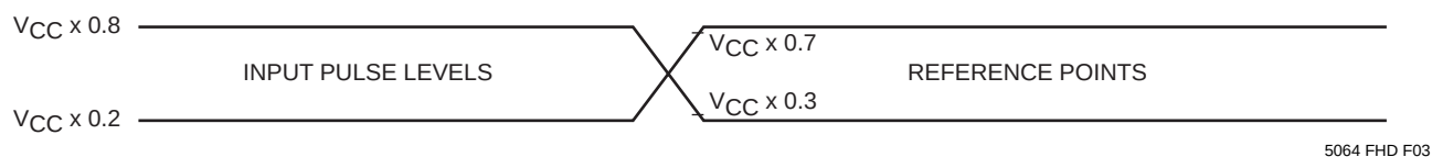
Figure 1. A.C. Testing Input/Output Waveform (2) (3) (4) ( C_L = 100 pF)
